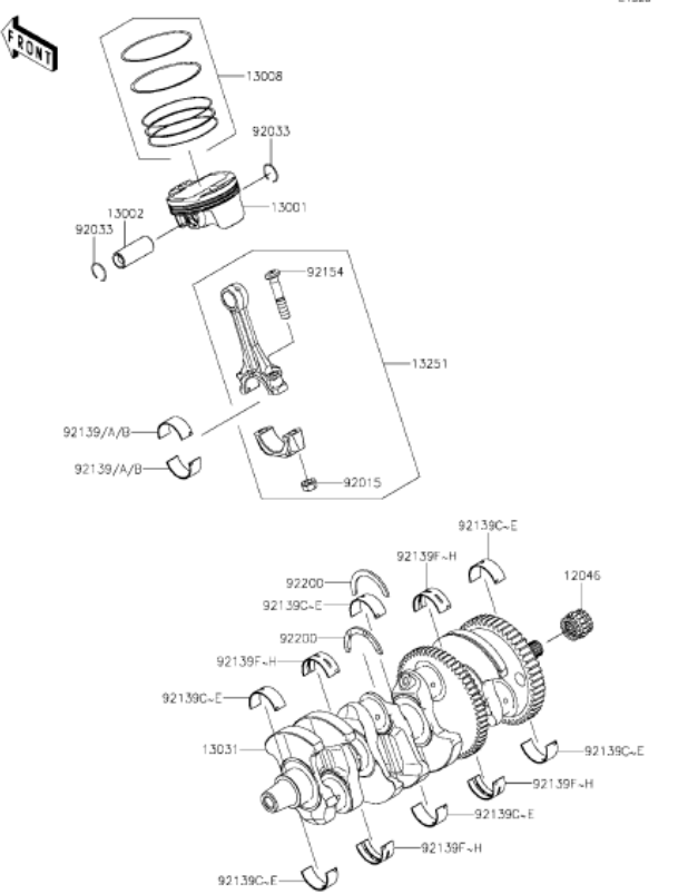
K7 Crankshaft/Piston(s)
