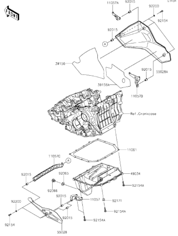
K16 Oil Pan
