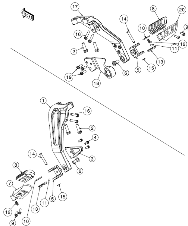
11.3 Passenger Footrests
