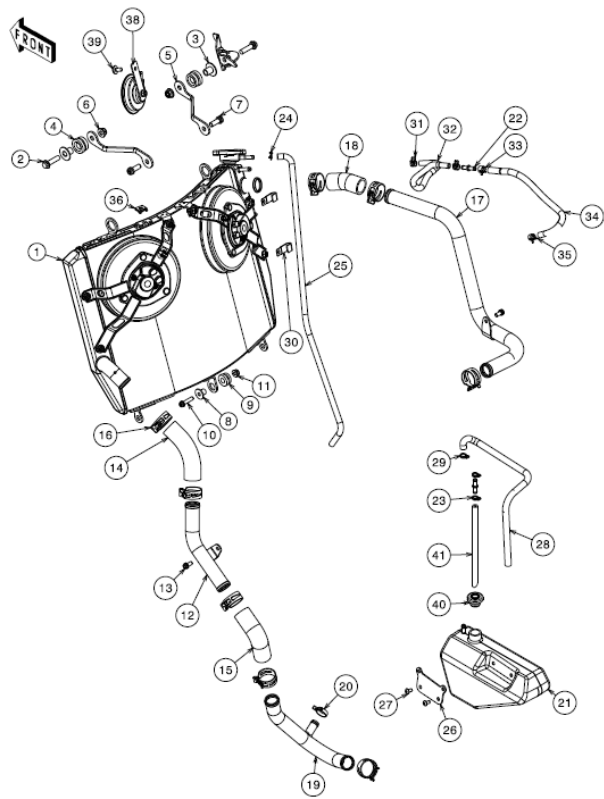
15 Cooling System
