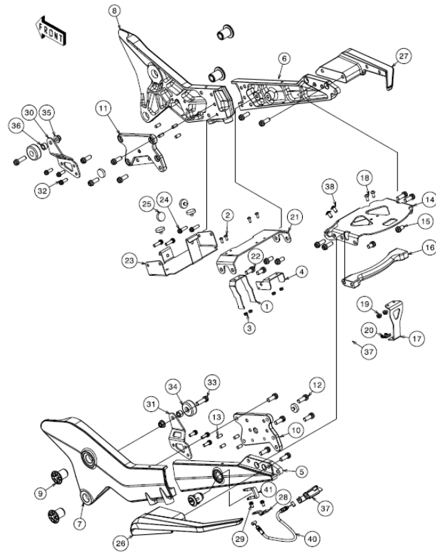
20 Tail Structure
