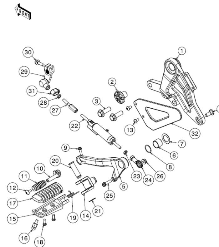
11.1 Footrest Left
