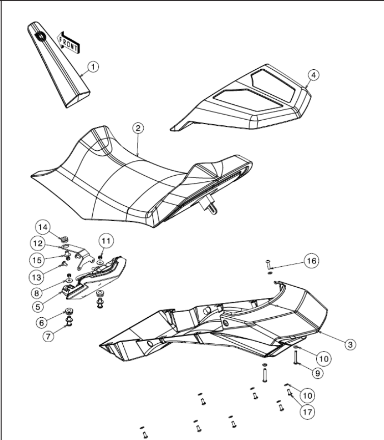
21.4 Tail Fairings Seats Lights
