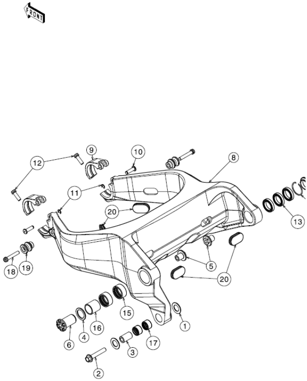
3.1 Front Swingarm
