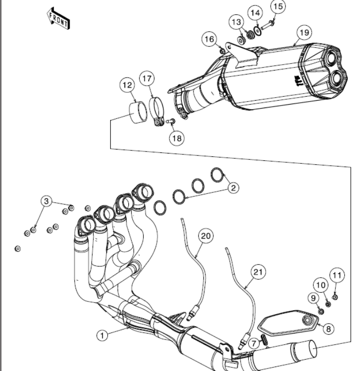
14 Hexhaust System
