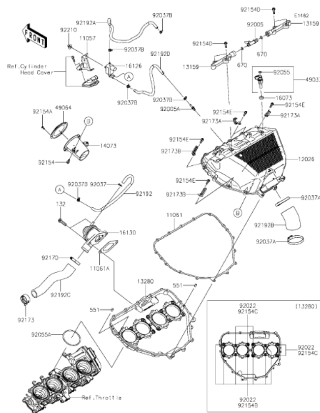
K18 Air Chamber
