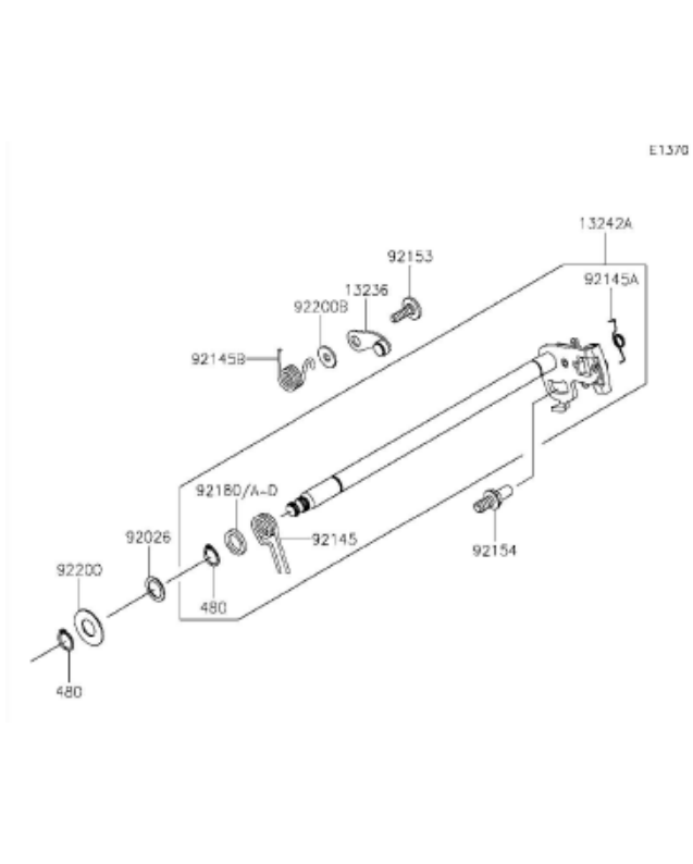
K12 Gear Change Mechanism
