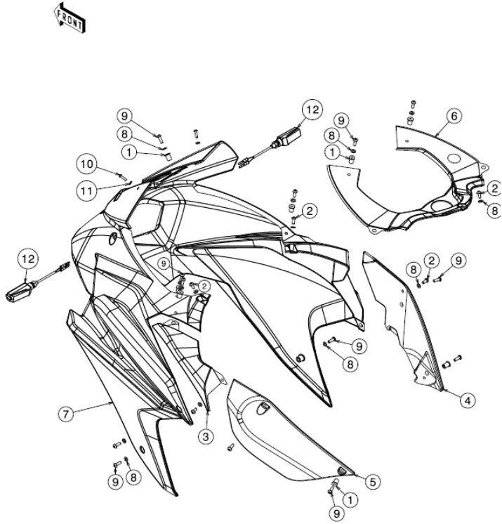
21.2 Front Fairing
