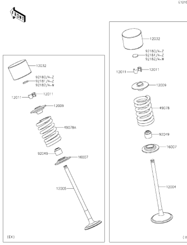
K5 Valves
