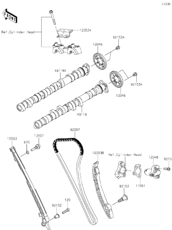
K6 Camshaft(s)/Tensioner
