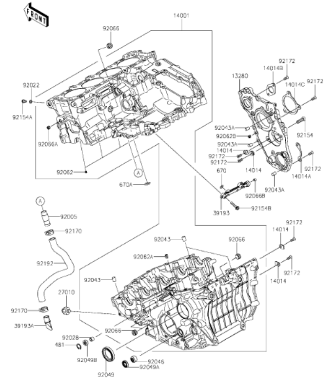
K13 Crankcase
