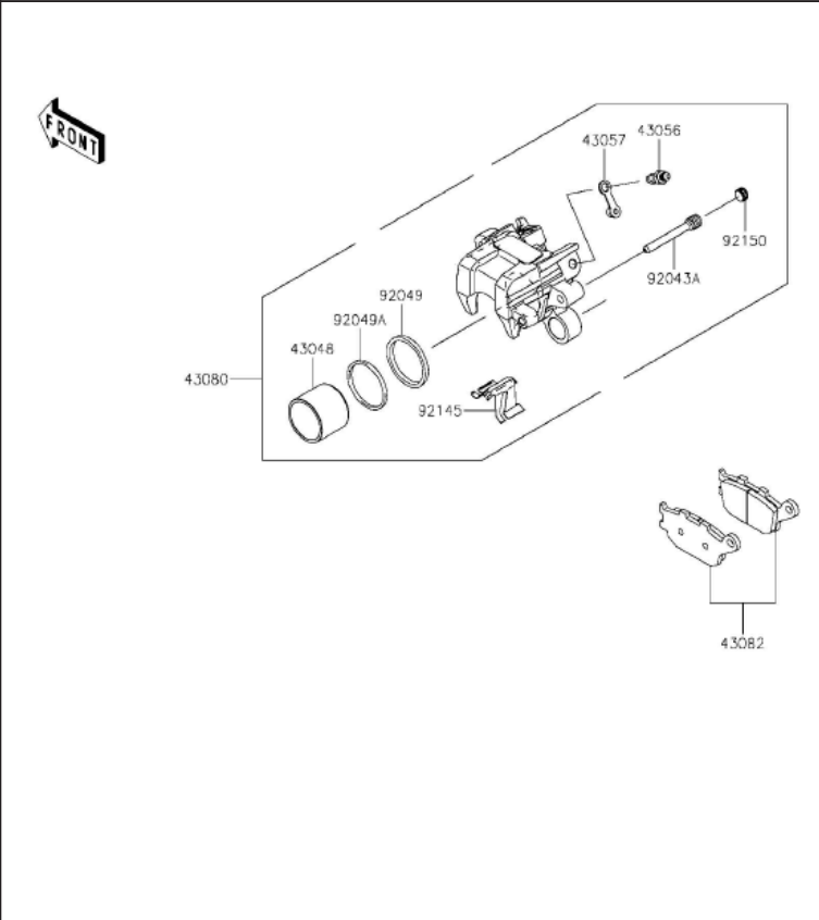
5.2 Caliper Sub Assy
