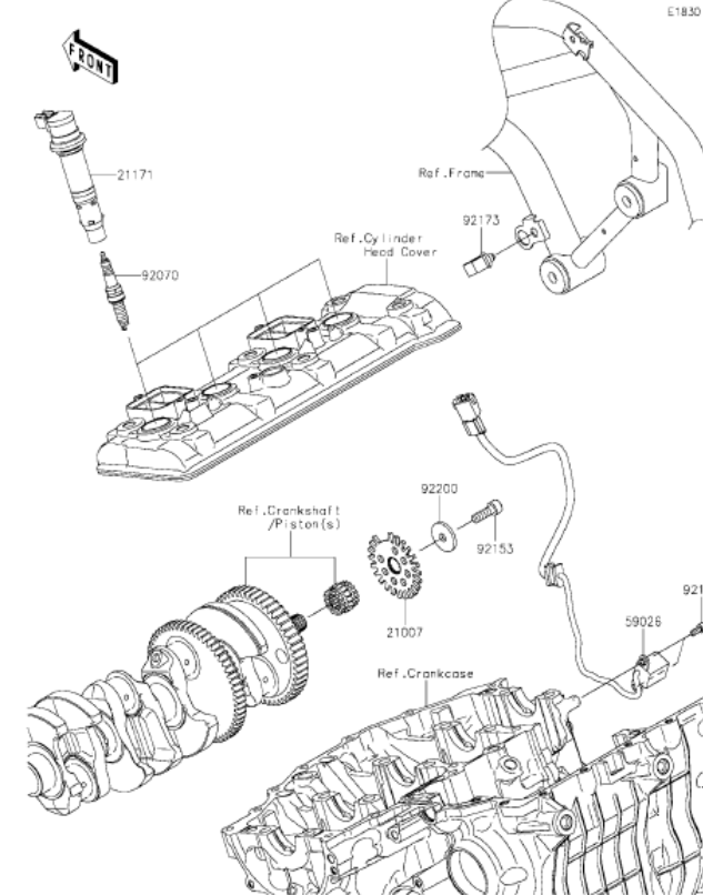
K25 Ignition System
