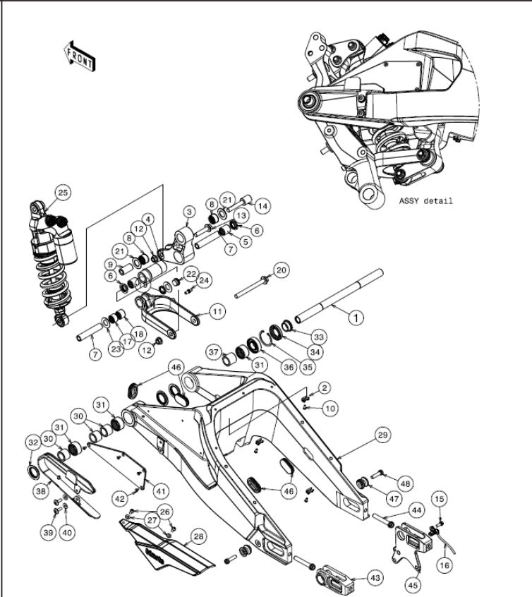
6 Rear Swingarm
