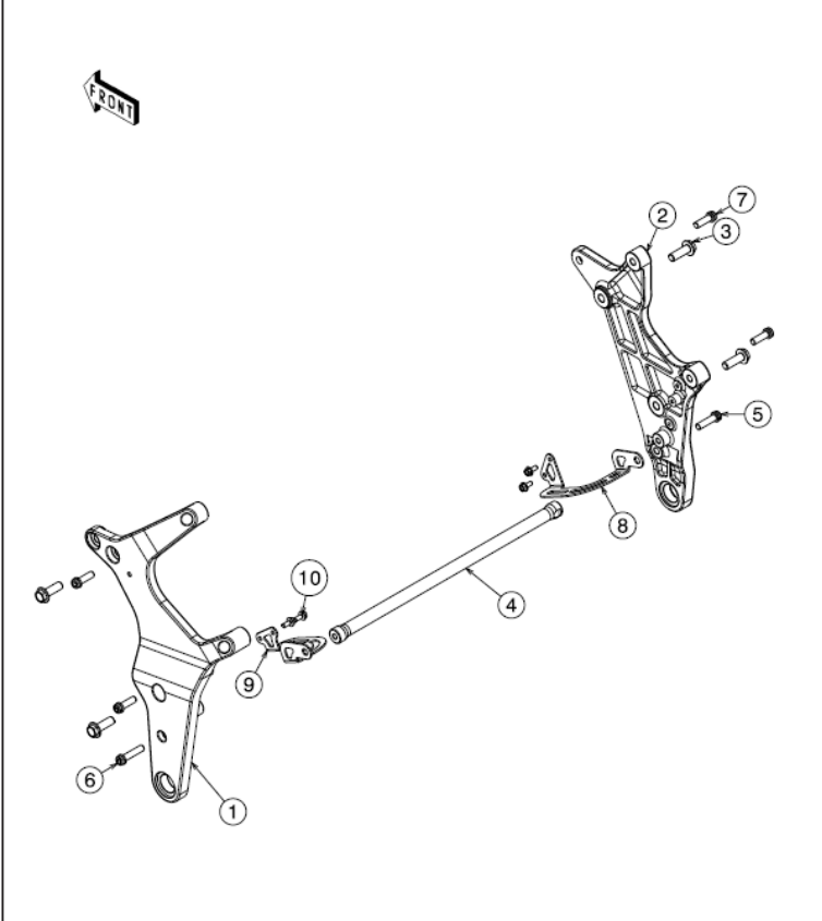
9.2 Frame Plates
