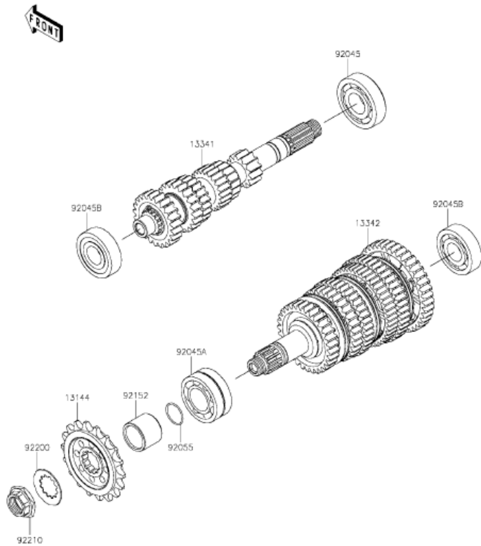
K10 Transmission
