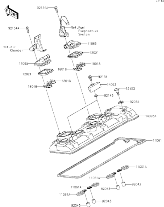
K2 Cylinder Head Cover
