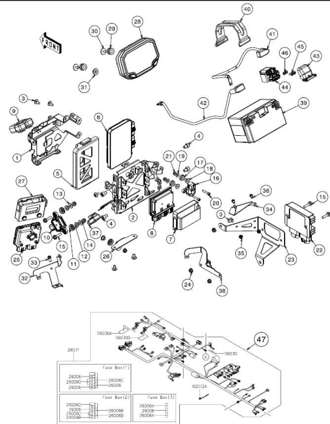
18 Electrical System
