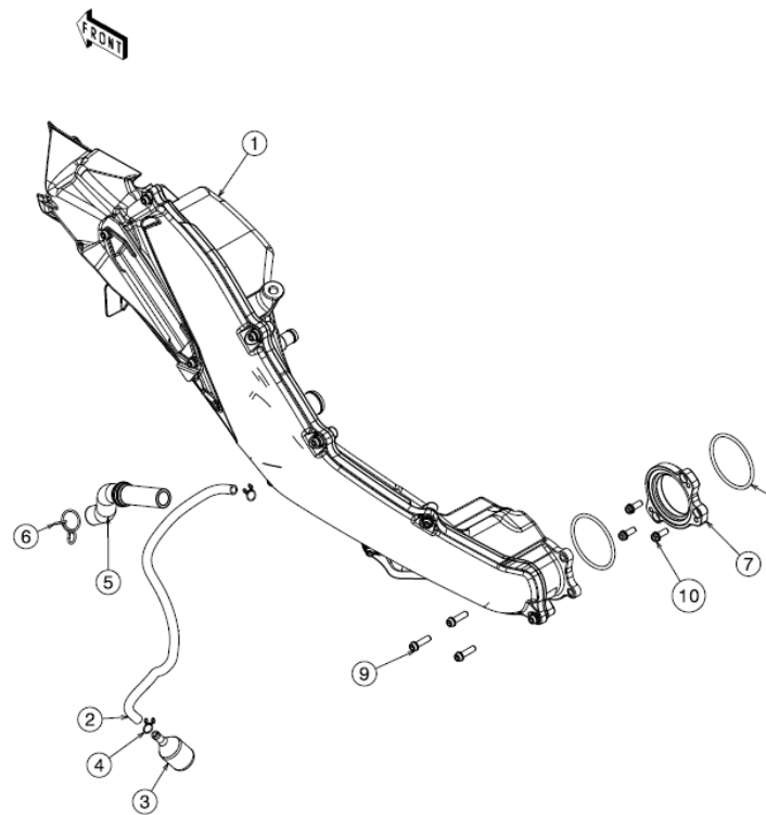
17 Airbox
