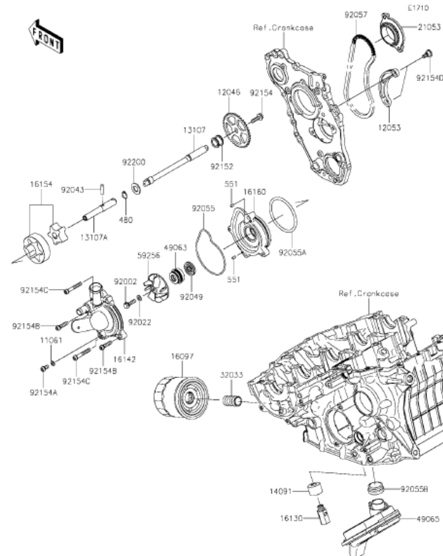
K23 Oil Pump
