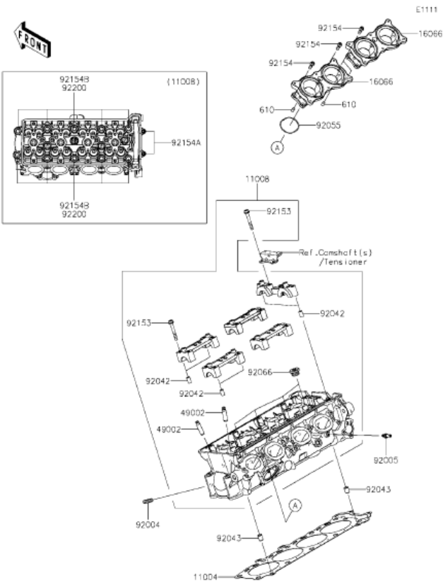
K1 Cylinder Head
