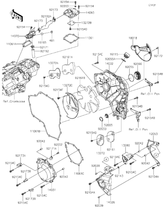
K15 Engine Cover(s)
