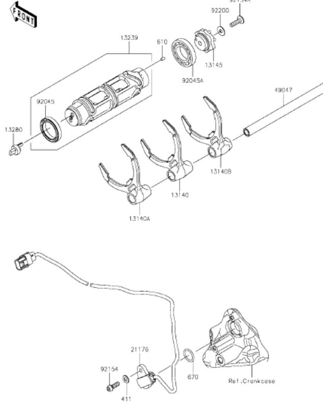
K11 Gear Change Drum/Shift Fork(s)
