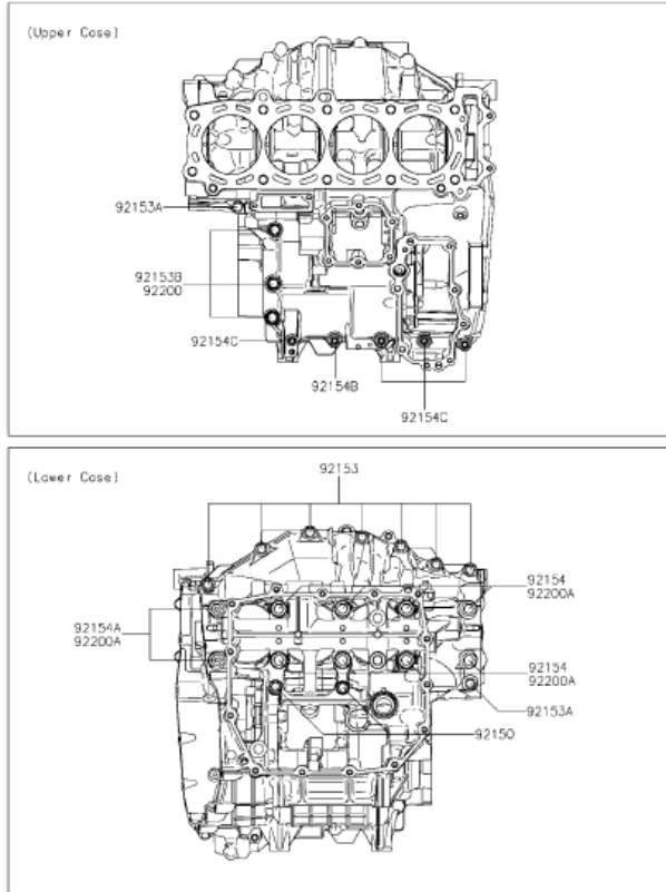
K14 Crankcase Bolt Pattern
