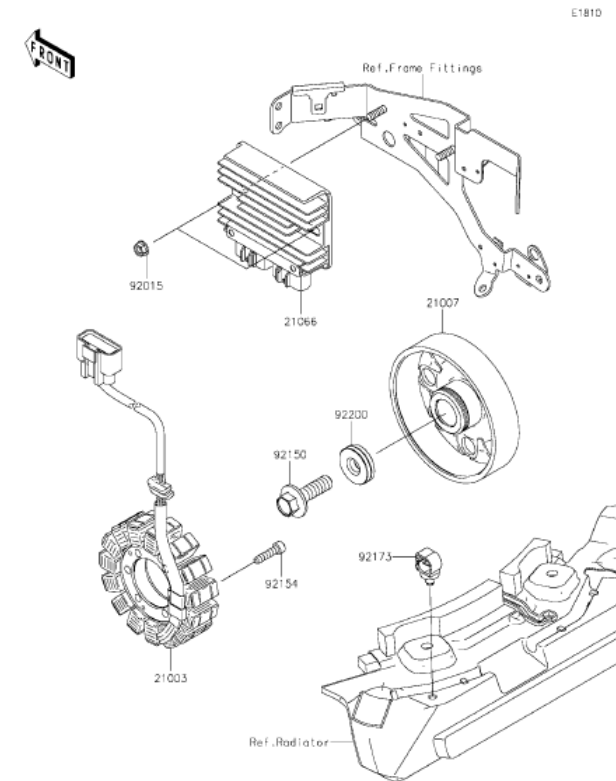
K24 Generator
