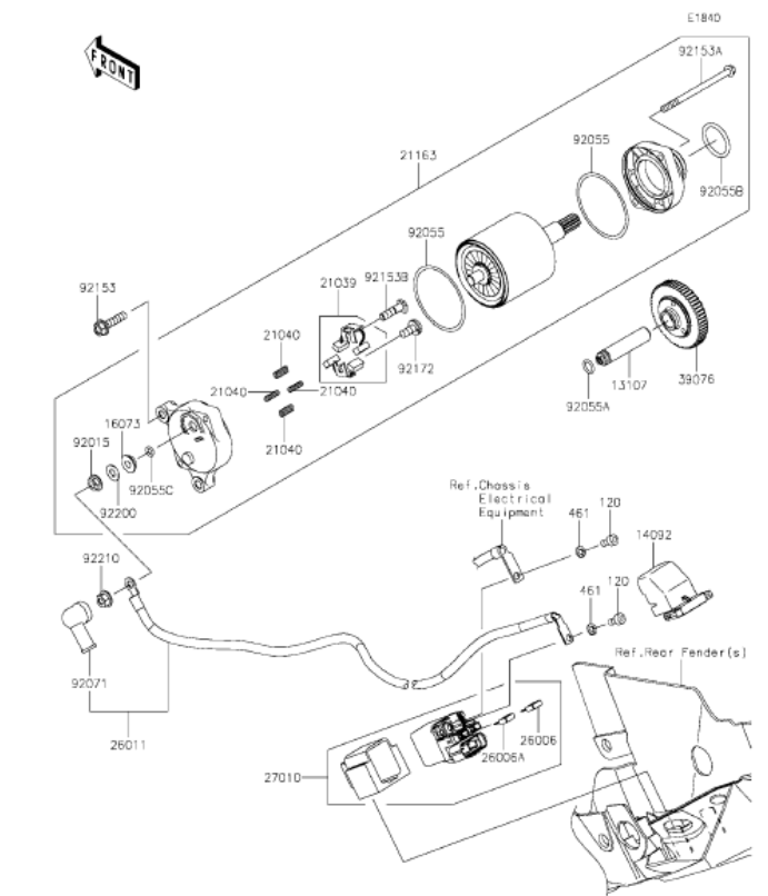
K26 Starter Motor
