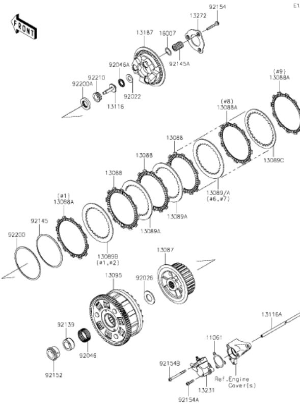
K9 Clutch
