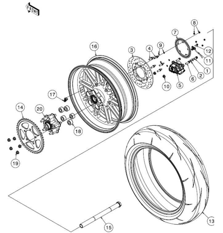
5.1 Rear wheel
