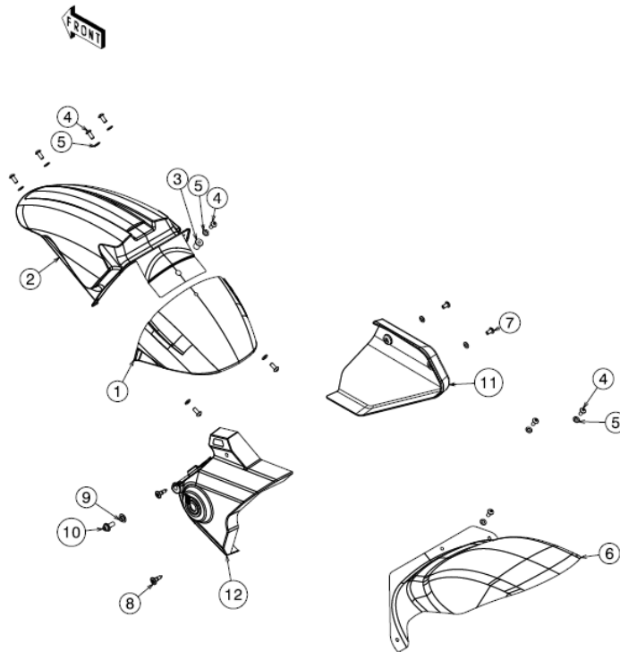
21.1 Fenders and Carbon Covers
