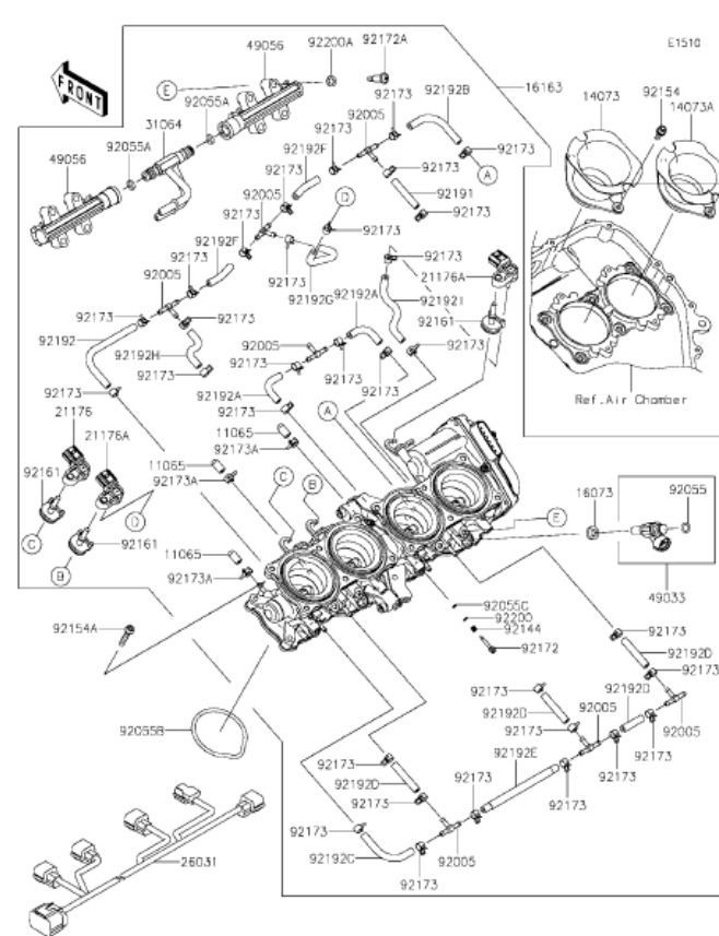
K19 Throttle
