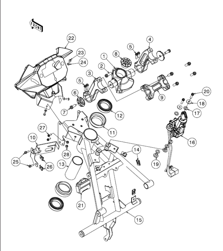
9.1 Front Frame w. Switch Assy
