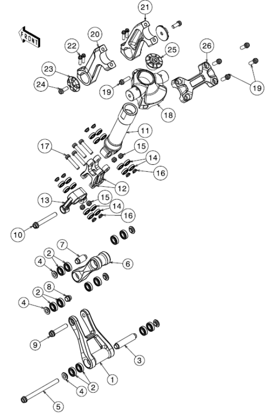
2 Steering linkage
