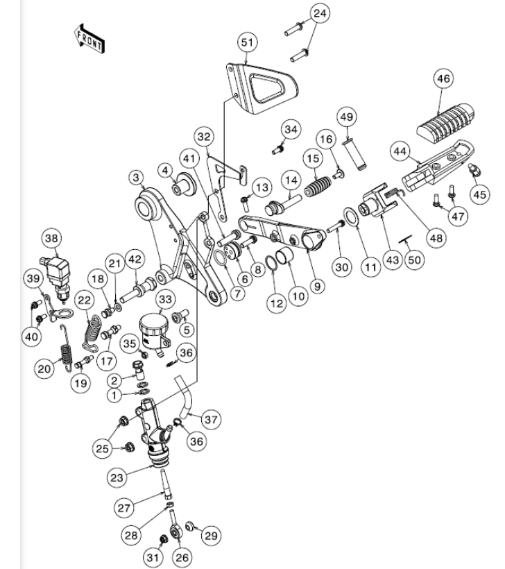
11.2 Footrest Right
