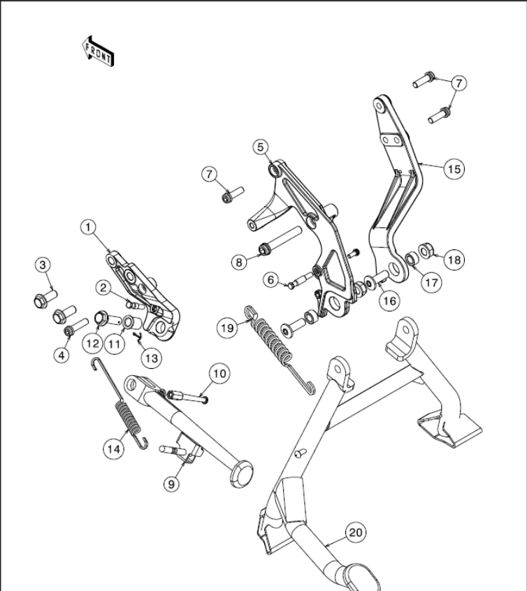
7 Stands
