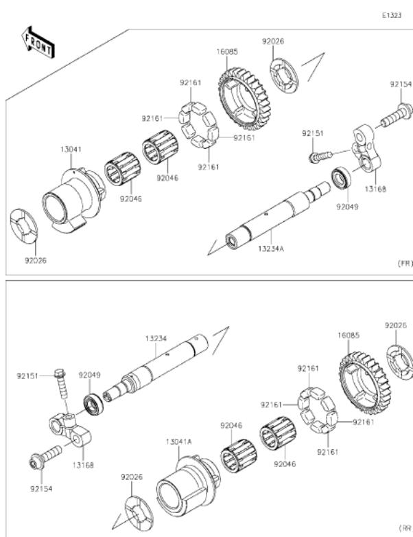
K8 Balancer
