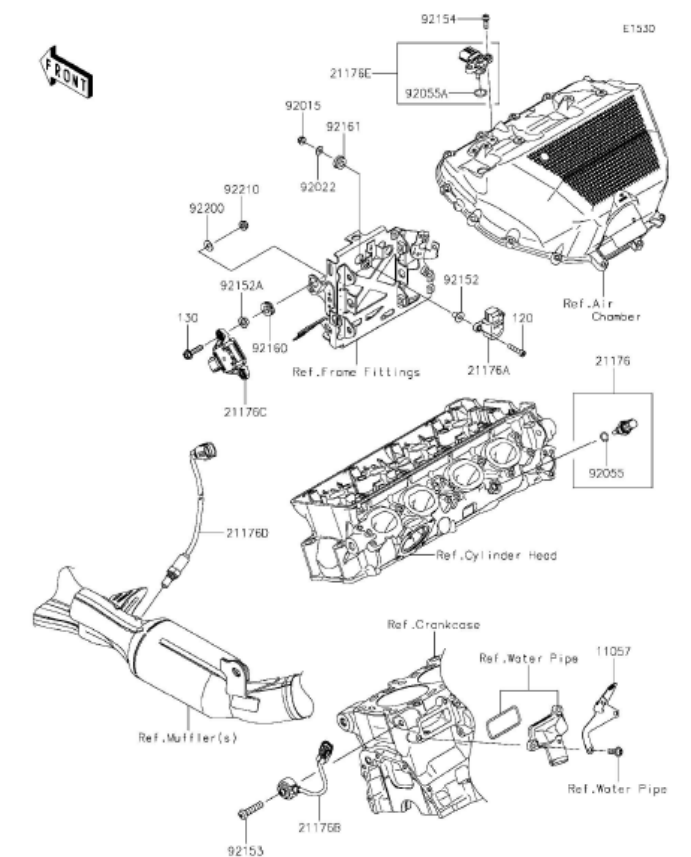
K21 Fuel Injection
