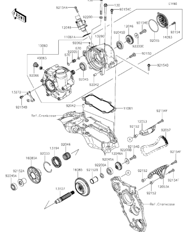
K17 Super Charger
