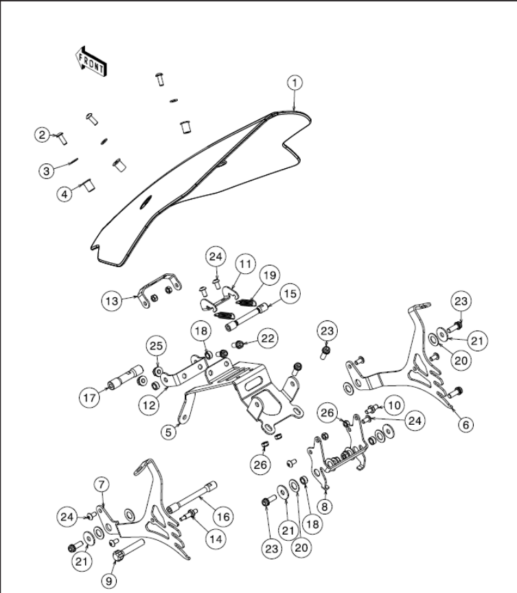
21.3 Windshield w. Adjuster Mechanism
