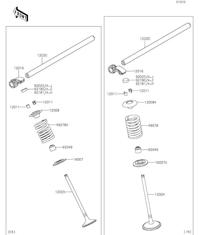
K5. Valves
