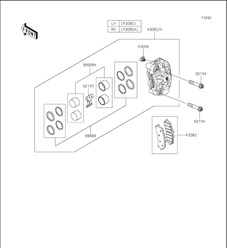
K43. Front Brake
