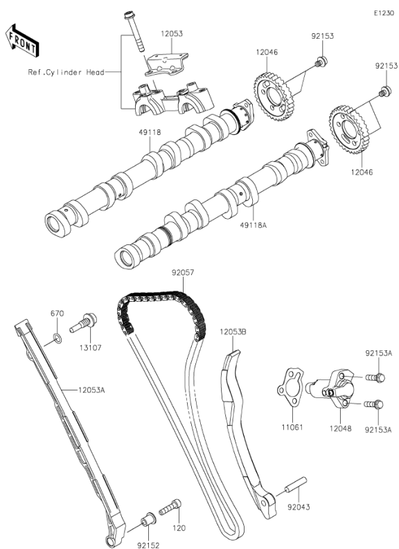
K6. Camshafts/Tensioner
