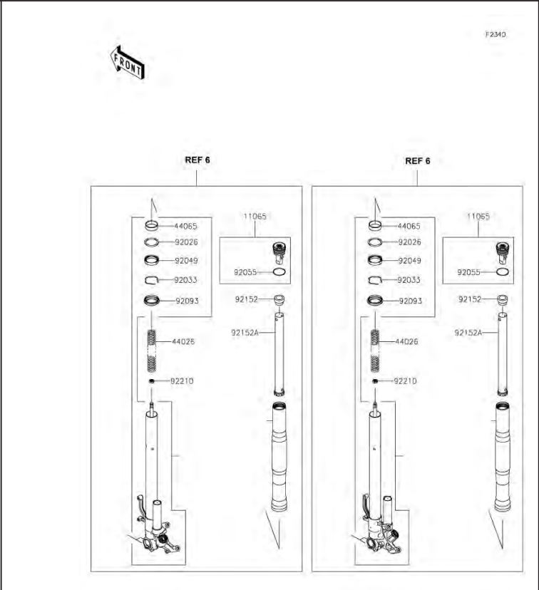
K48. Front Fork
