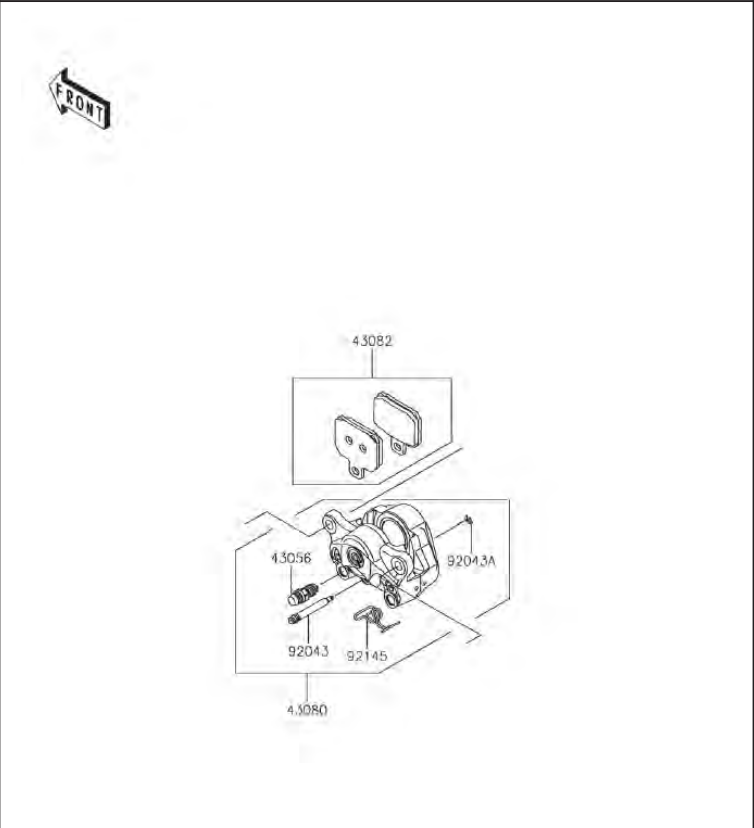
K45. Rear Brake Caliper ASSY
