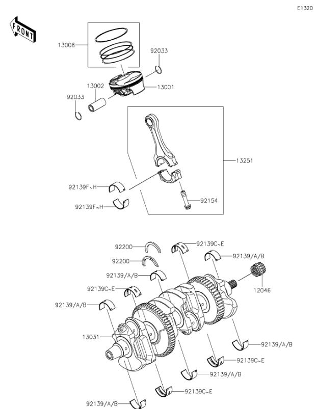
K7. Crankshaft/Pistons
