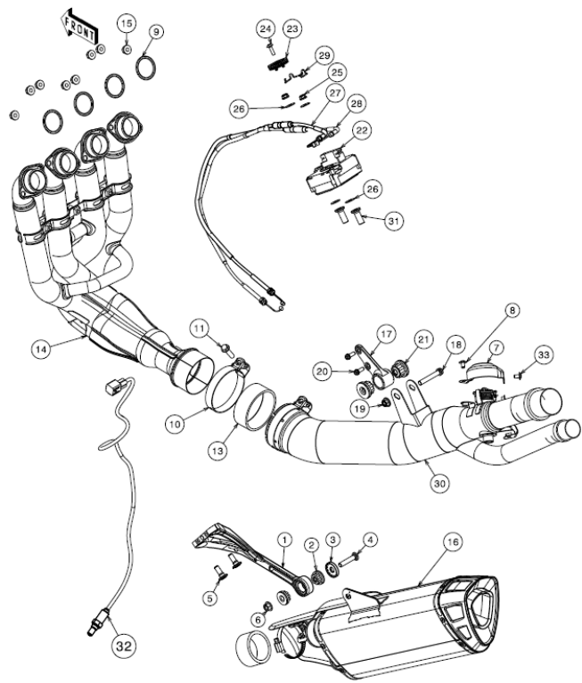
5. Exhaust system
