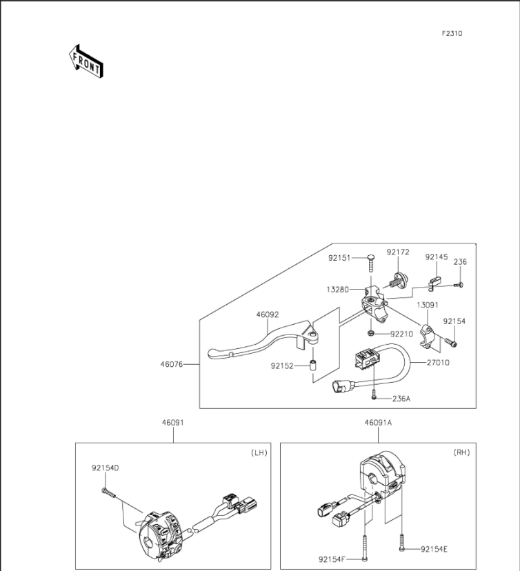
K46. Handlebar
