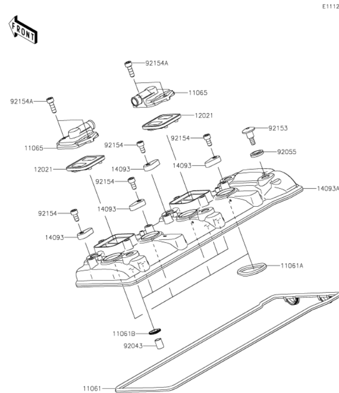
K2. Cylinder head cover
