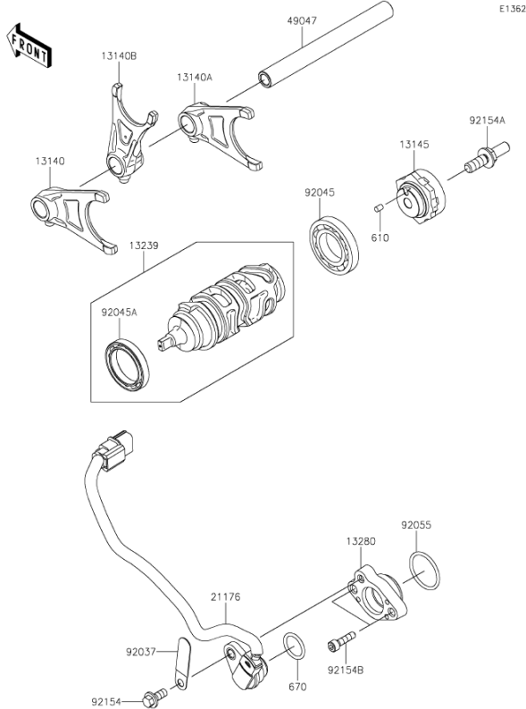
K11. Gear change Drum/Shift Forks
