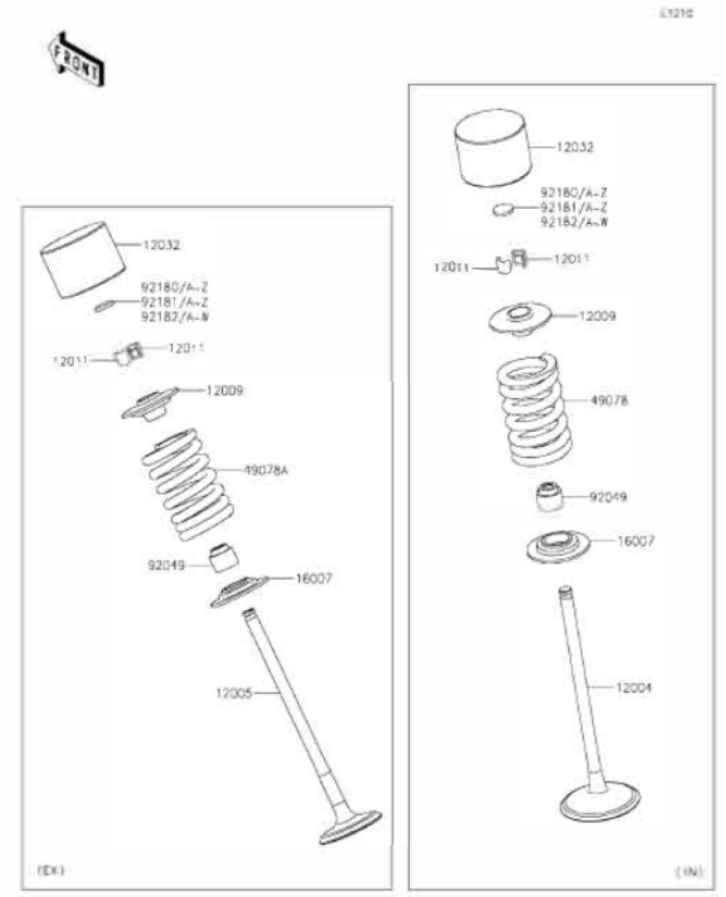
K5 Valves
