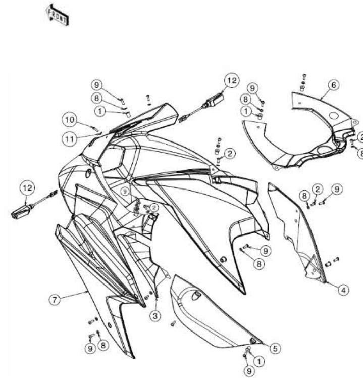
21.2 Front Fairing
