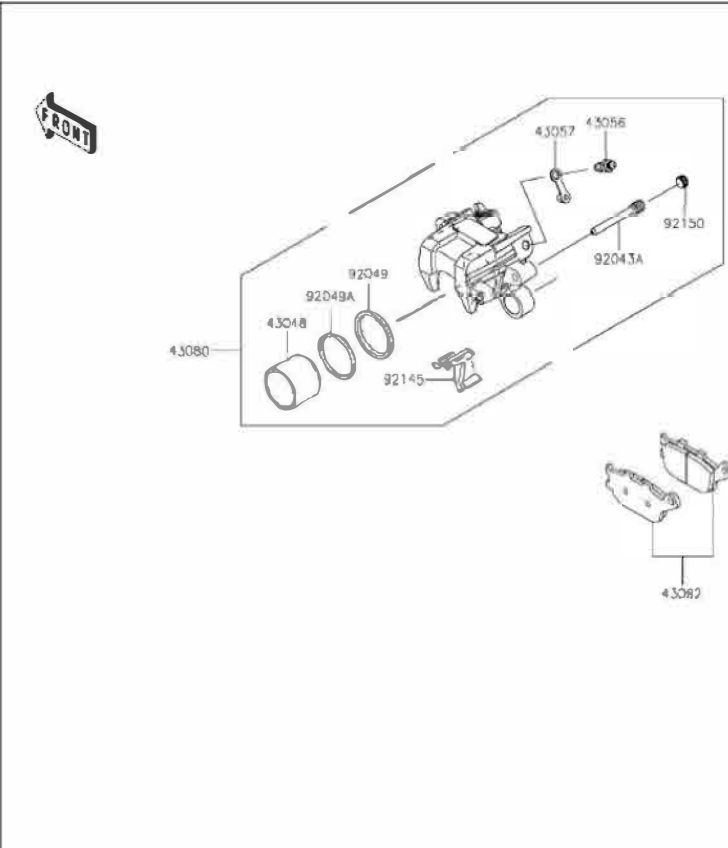
5.2 Caliper Sub Assy
