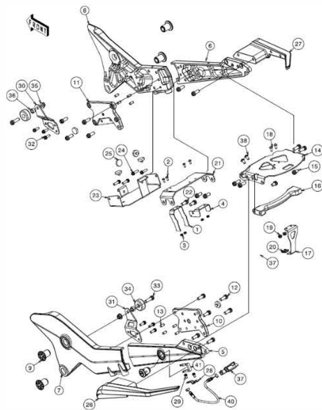
20 Tail Structure
