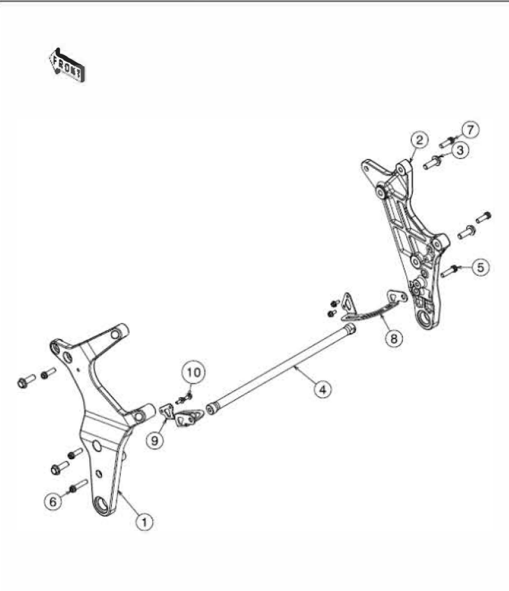
9.2 Frame Plates
