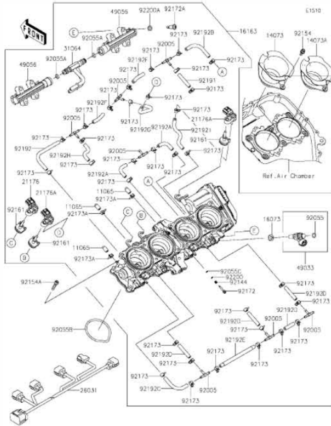
K19 Throttle
