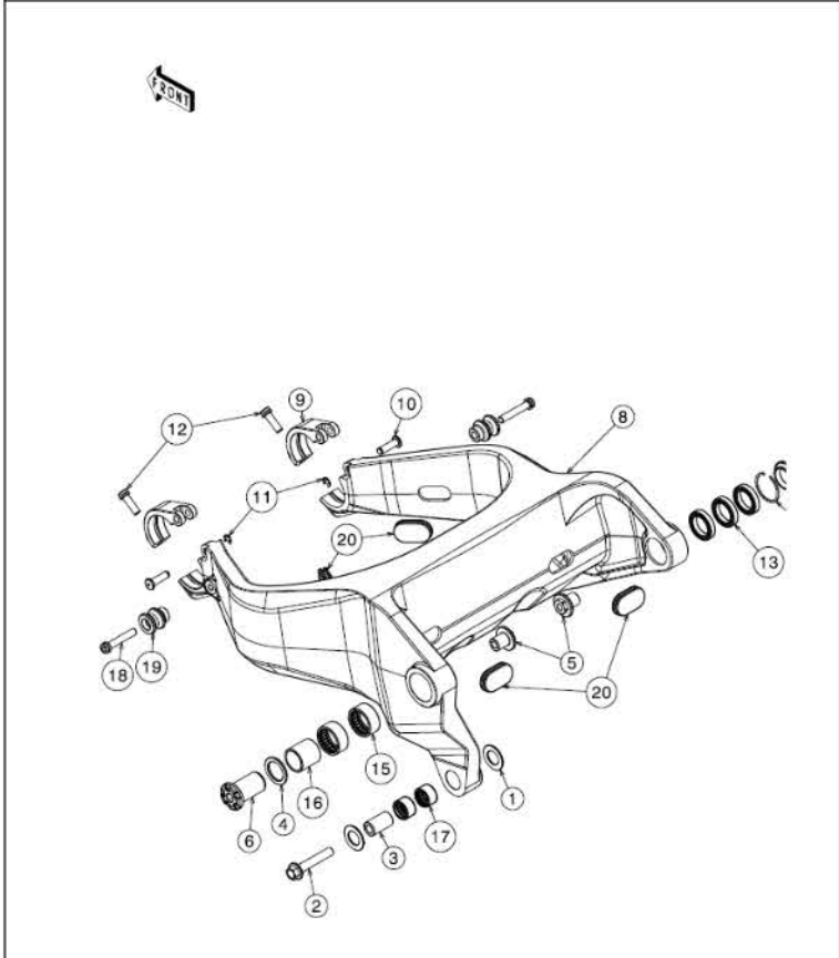
3.1 Front Swingarm
