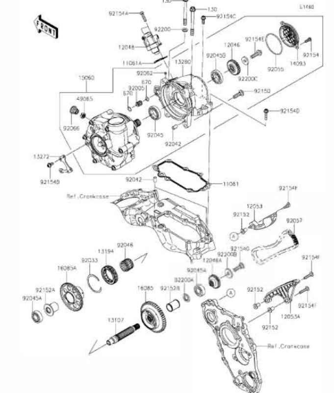
K17 Super Charger
