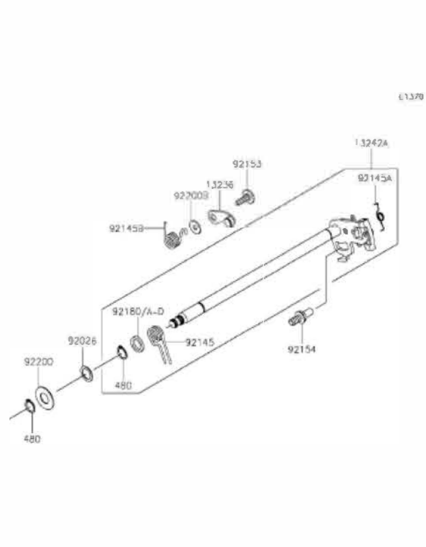
K12 Gear Change Mechanism
