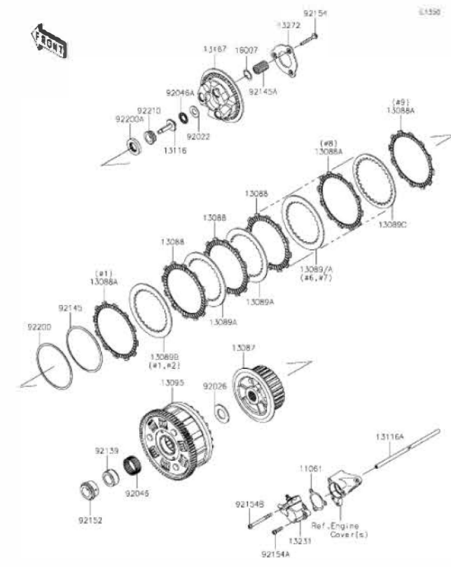
K9 Clutch
