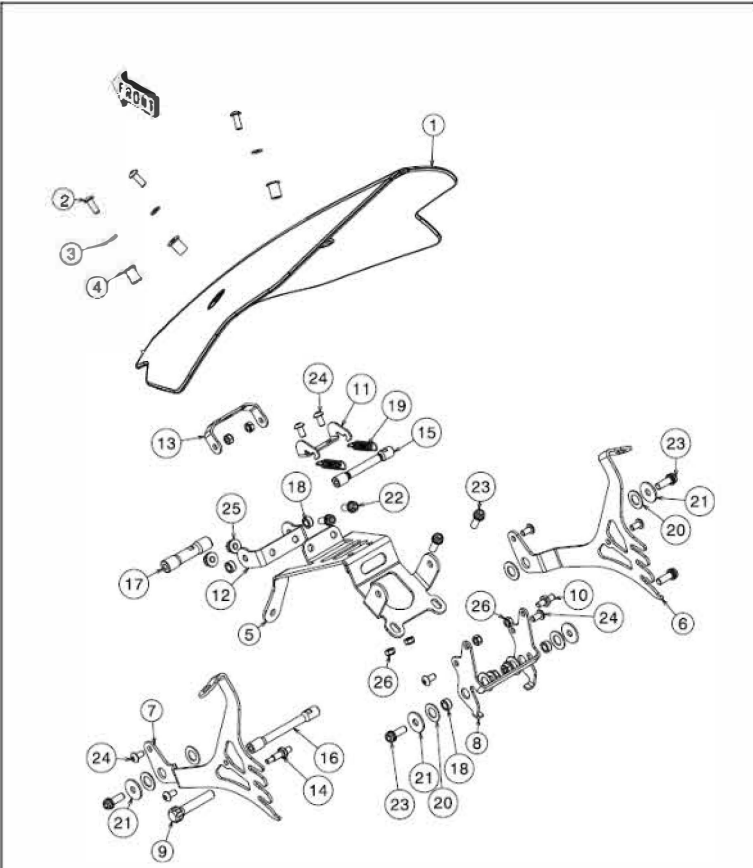
21.3 Windshield w. Adjuster Mechanism
