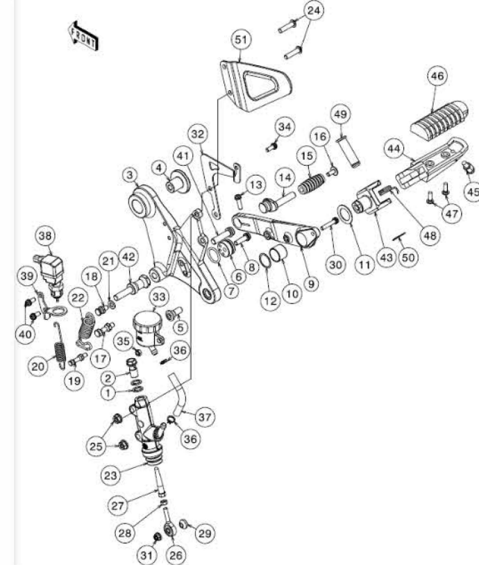
11.2 Footrest Right
