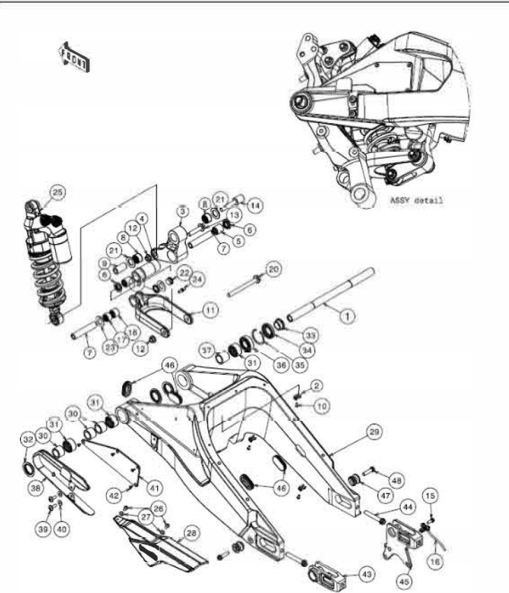
6 Rear Swingarm
