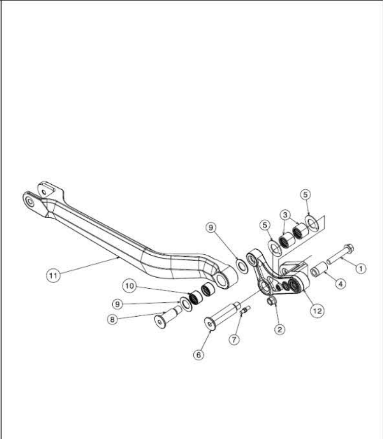
3.2 Front Suspension linkage
