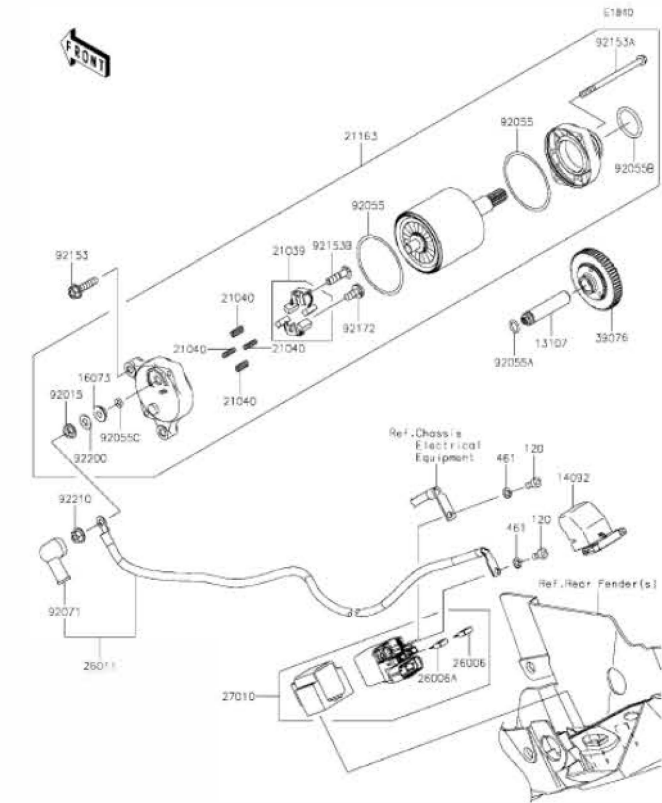
K26 Starter Motor
