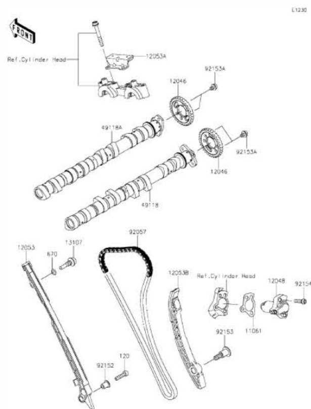
K6 Camshaft(s)/Tensioner
