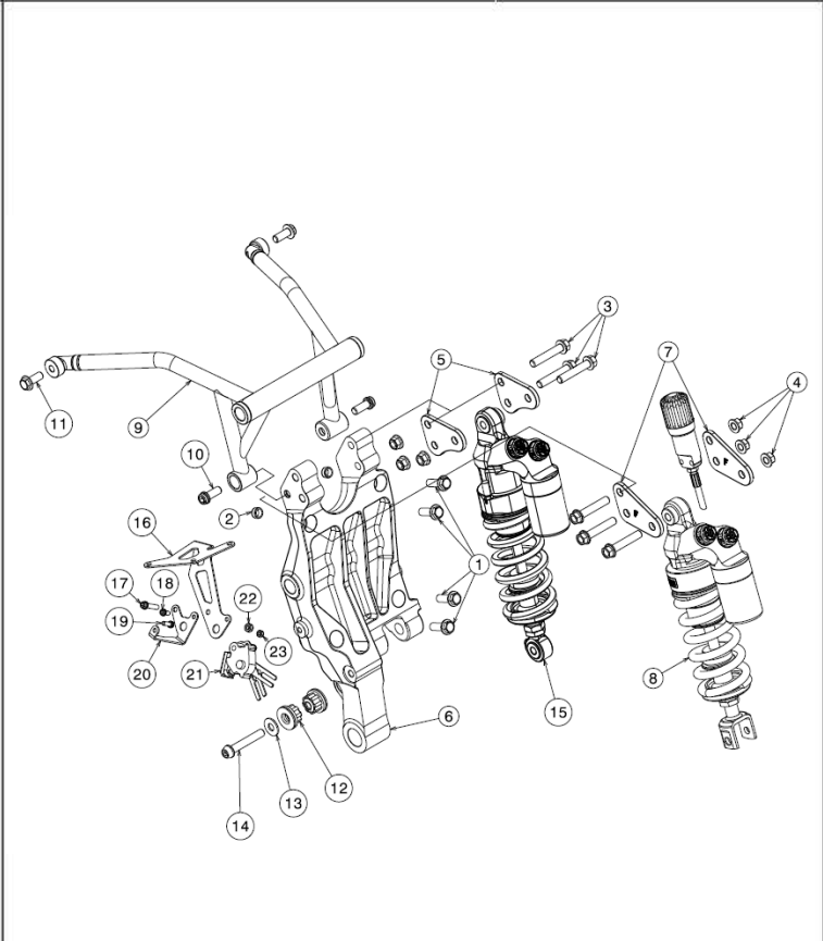
4 Rear structure . shockabsorbers
