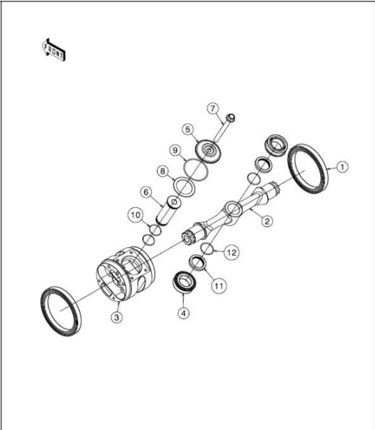
1.2 Front Hub
