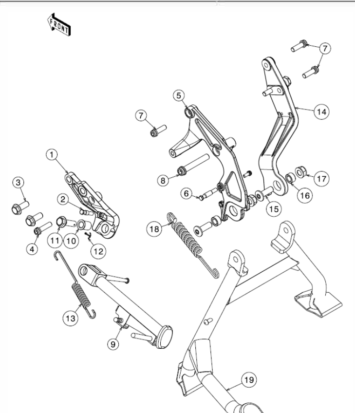
7 Stands
