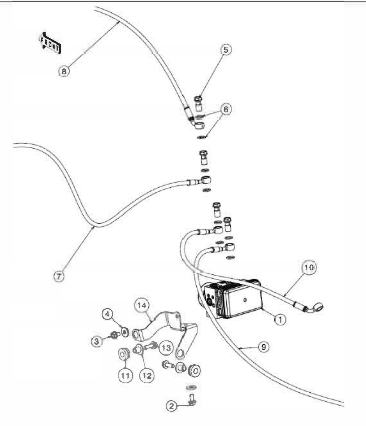
8 ABS unit w. Pipes
