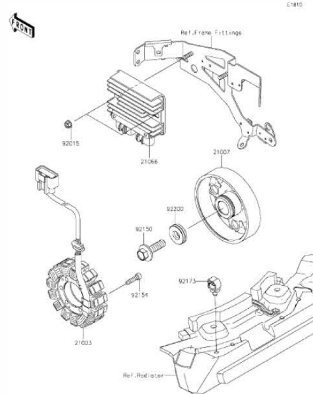
K24 Generator
