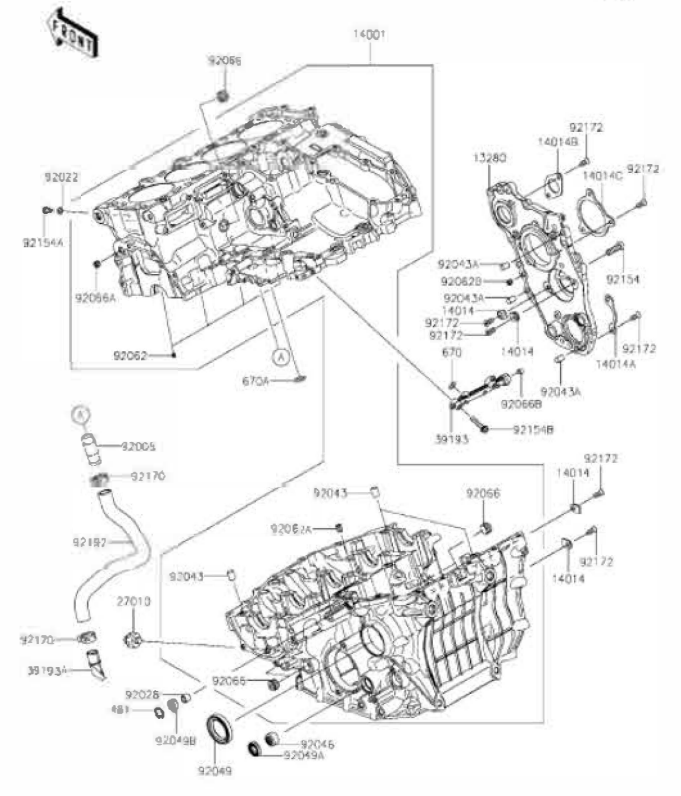
K13 Crankcase
