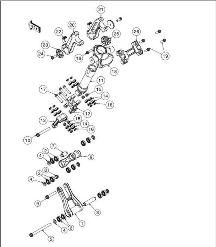
2 Steering linkage
