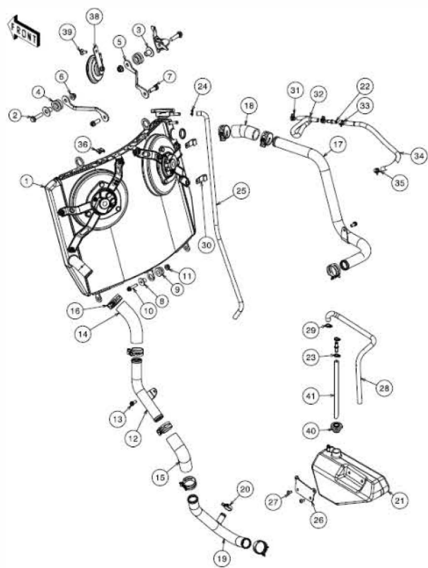
15 Cooling System
