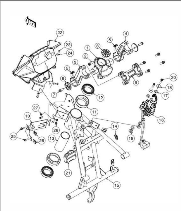
9.1 Front Frame w. Switch Assy
