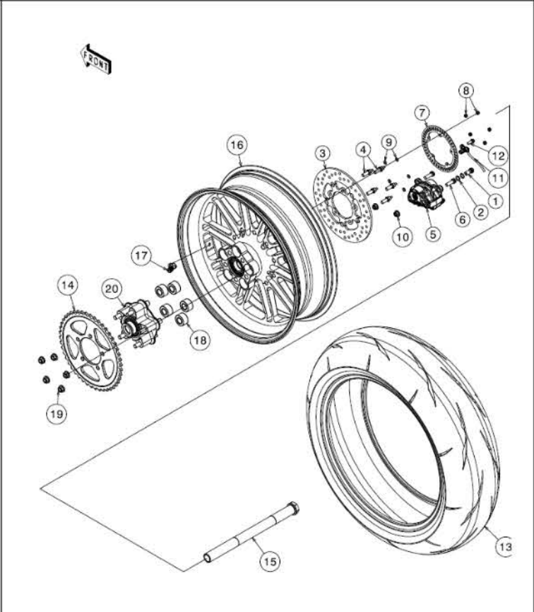
5.1 Rear wheel
