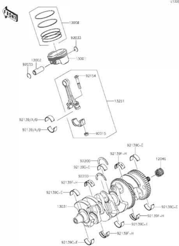
K7 Cranckshaft/Piston(s)
