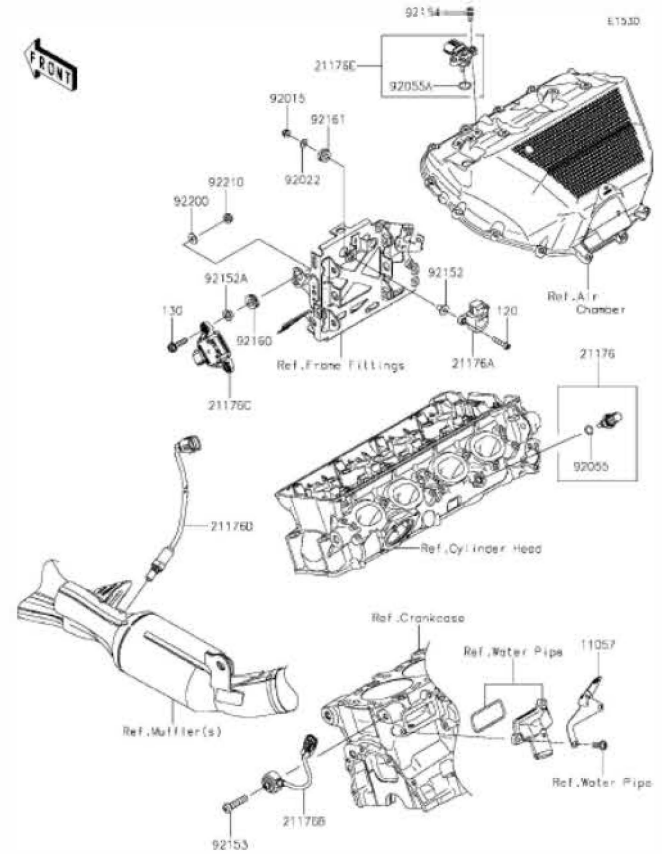
K21 Fuel Injection
