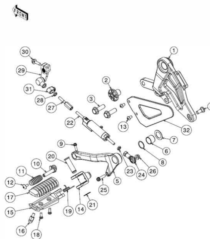
11.1 Footrest Left
