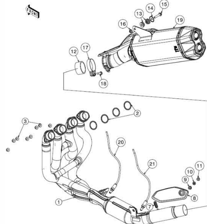
14 Hexhaust System
