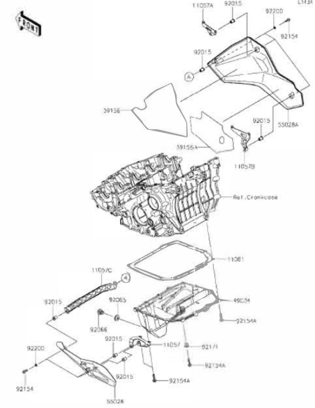
K16 Oil Pan
