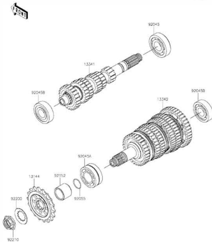
K10 Transmission
