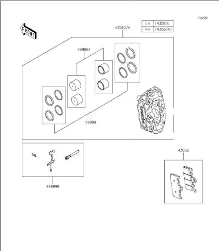
1.3 Caliper Sub Assy
