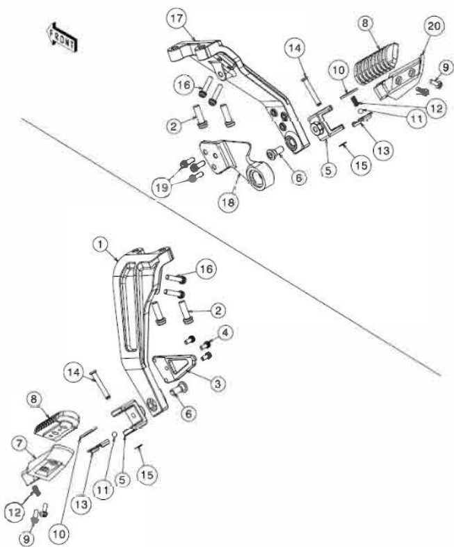
11.3 Passenger Footrests
