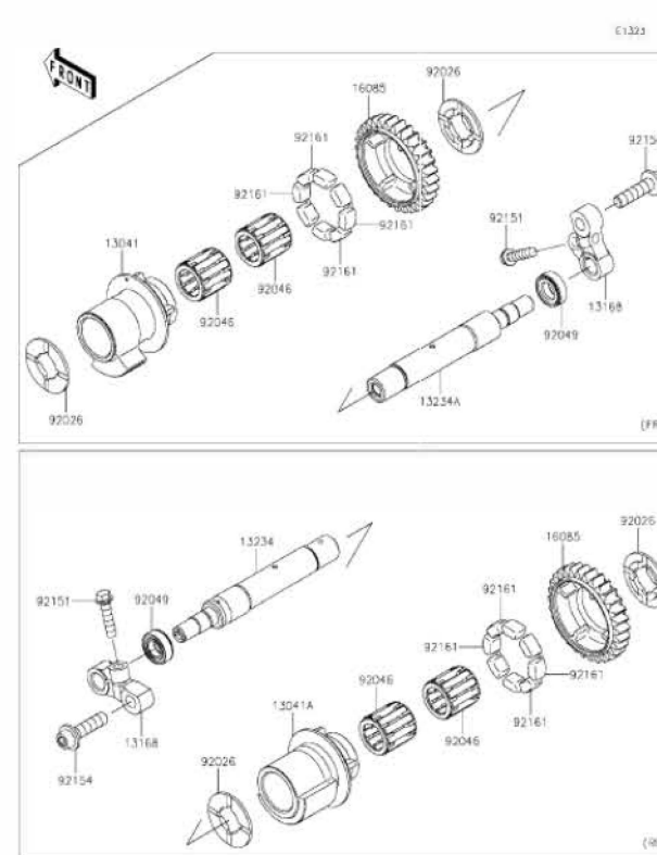
K8 Balancer
