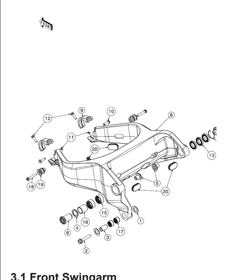
3.1 Front Swingarm
