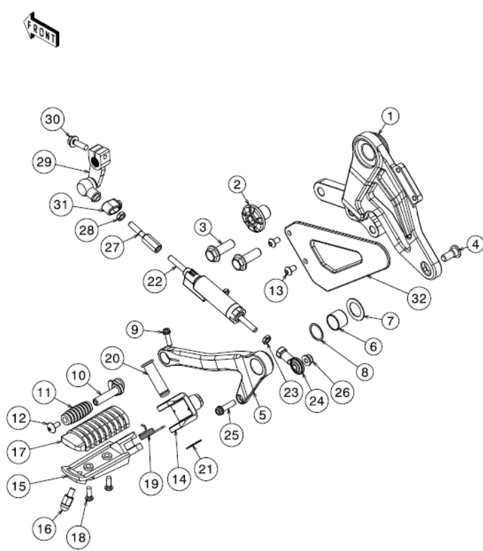
11.1 Footrest Left
