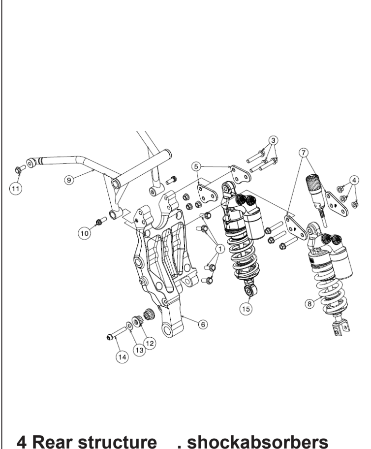
4 Rear structure . shockabsorbers
