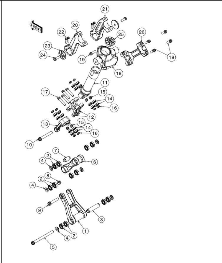
2 Steering linkage
