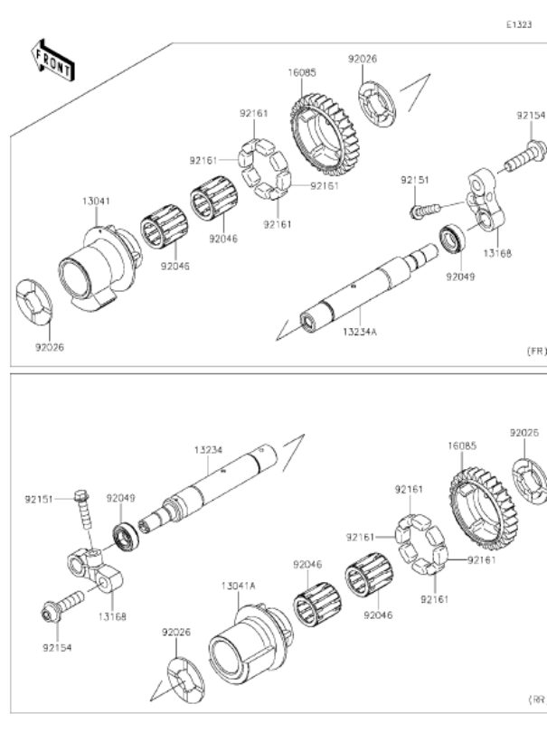
K8 Balancer
