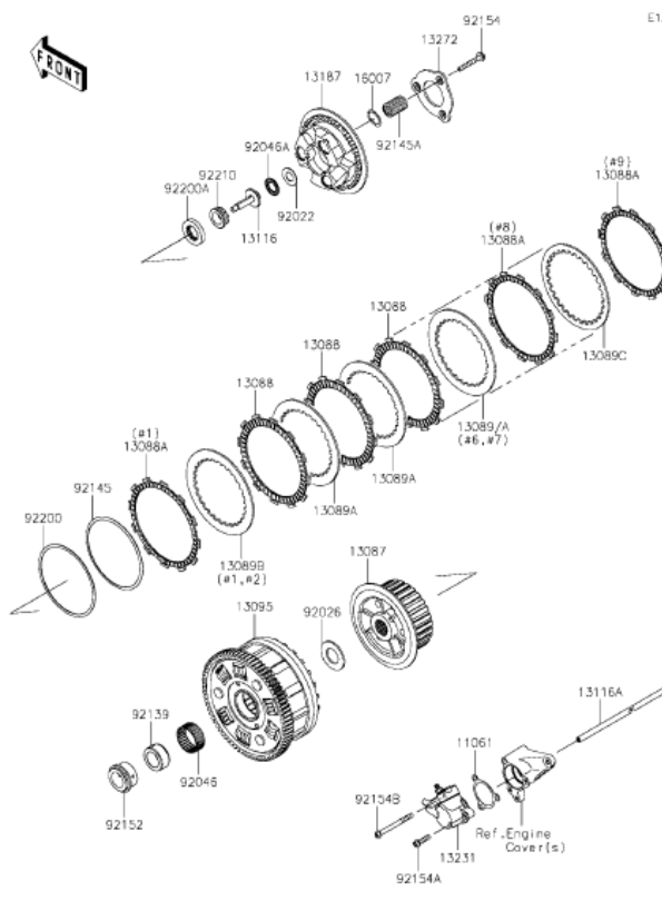
K9 Clutch
