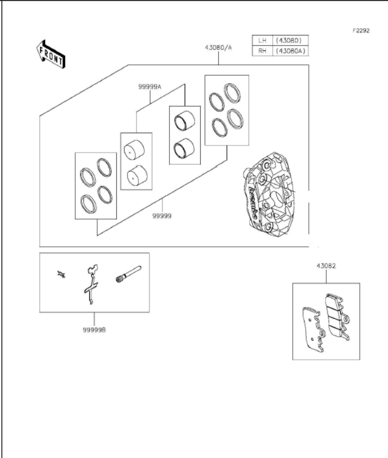
1.3 Caliper Sub Assy
