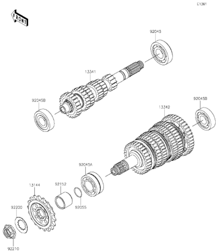
K10 Transmission
