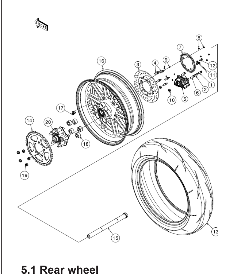
5.1 Rear wheel
