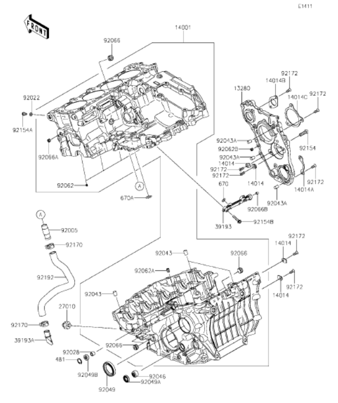
K13 Crankcase
