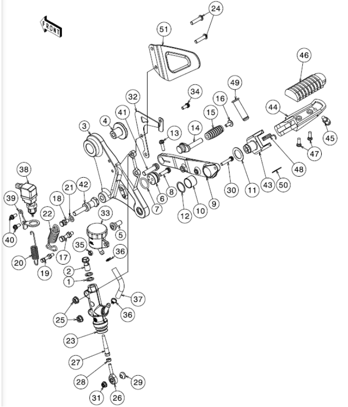
11.2 Footrest Right
