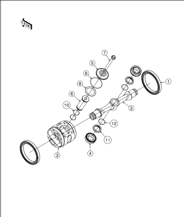
1.2 Front Hub
