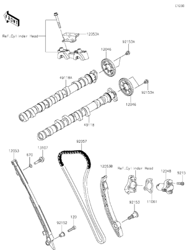
K6 Camshaft(s)/Tensioner
