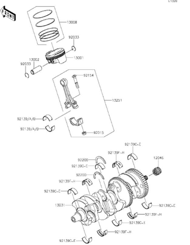
K7 Crankshaft/Piston(s)
