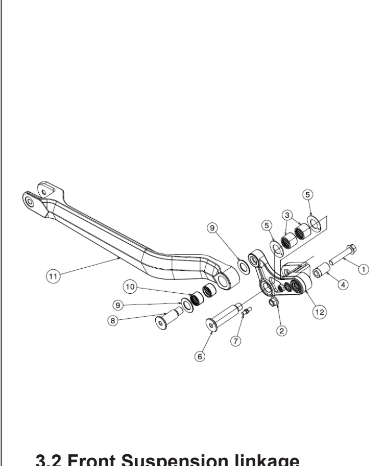
3.2 Front Suspension linkage
