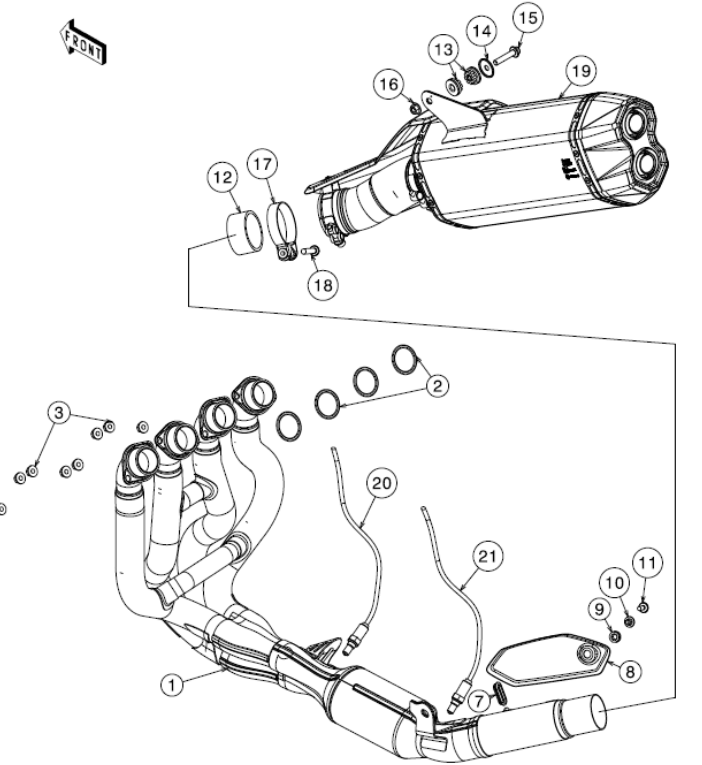
14 Hexhaust System
