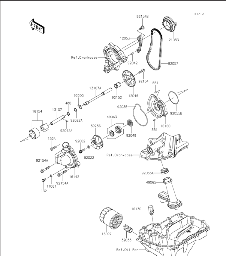
K21. Oil Pump
