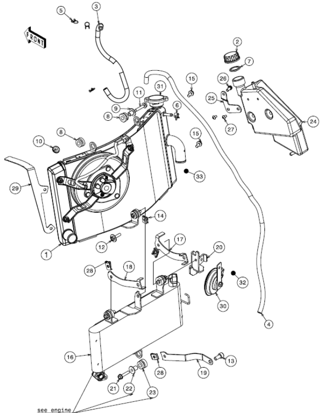
4. Cooling system
