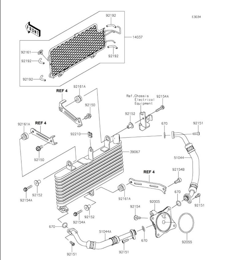
K26. Oil Cooler
