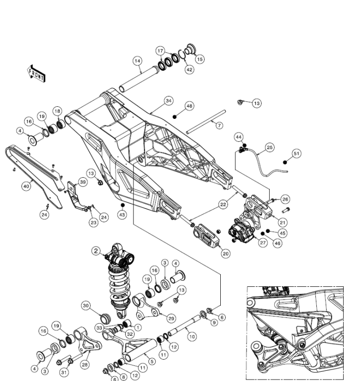
3. Rear swingarm
