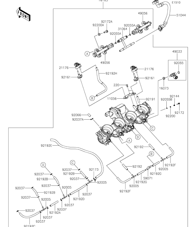
K17. Throttle
