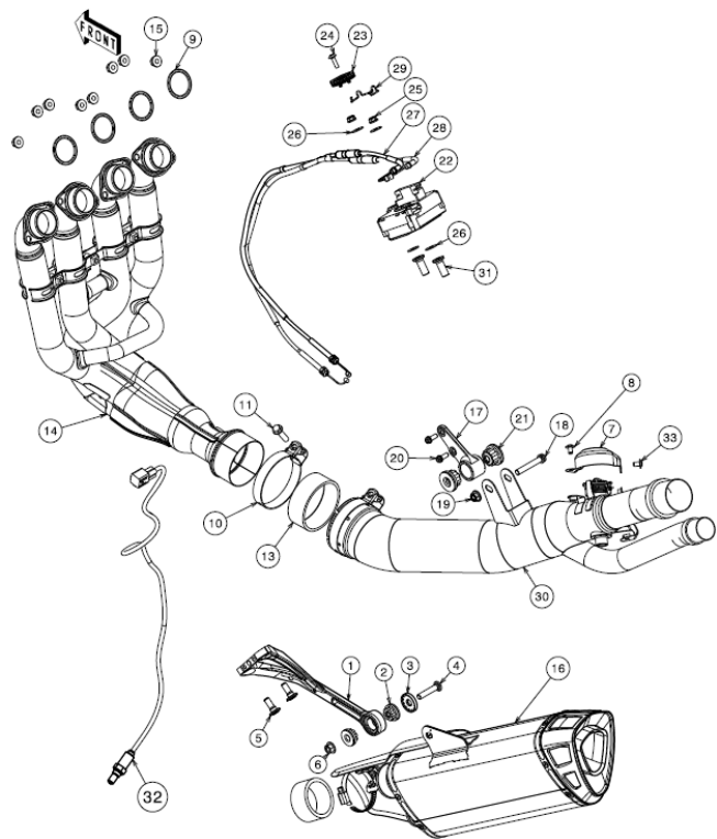
5. Exhaust system
