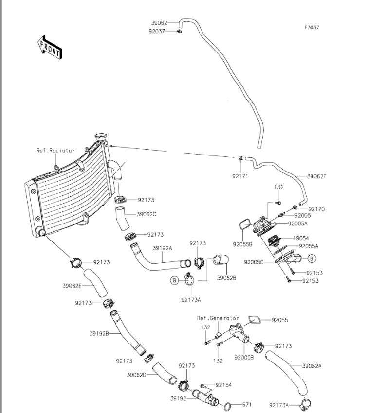
K27. Water Pipe
