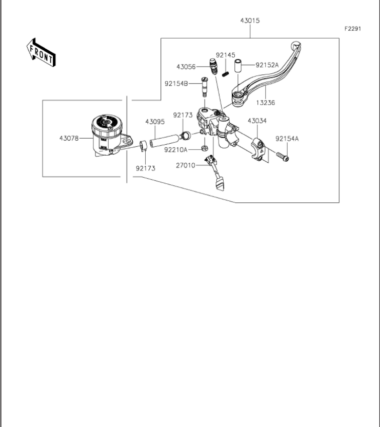
K42. Front master Cylinderch
