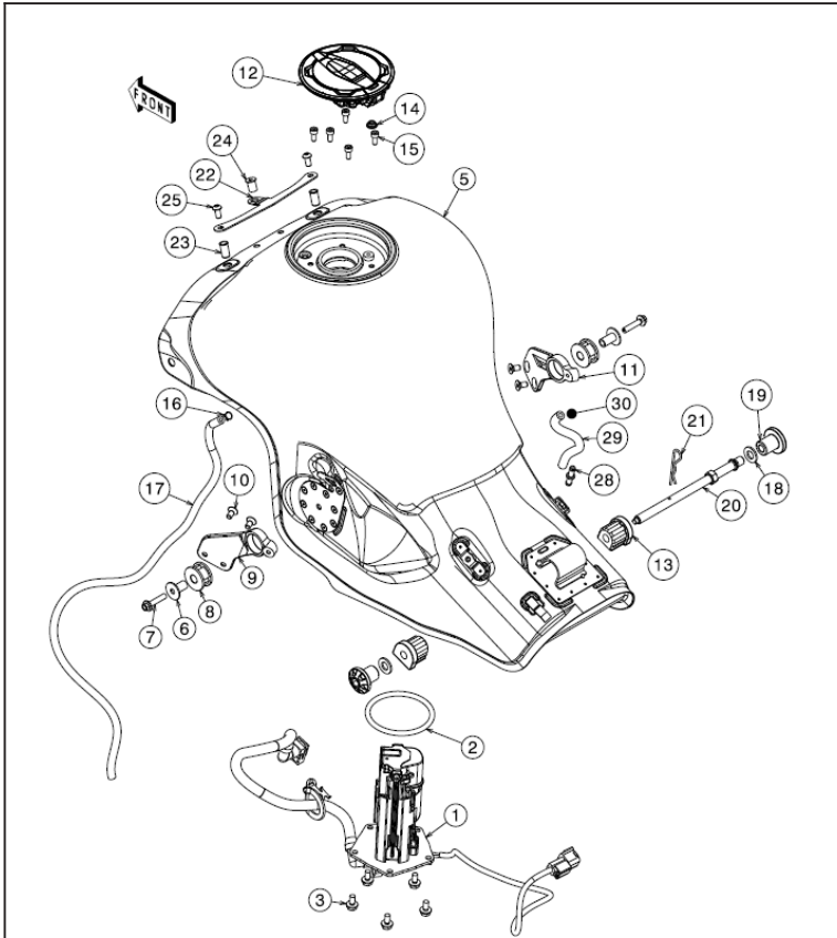
17. Fuel tank
