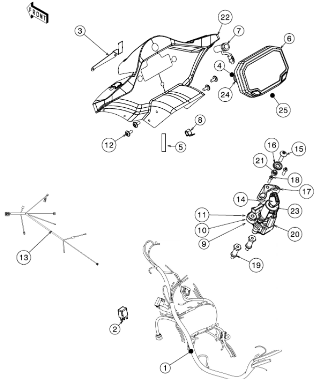
7. Electric system (main)
