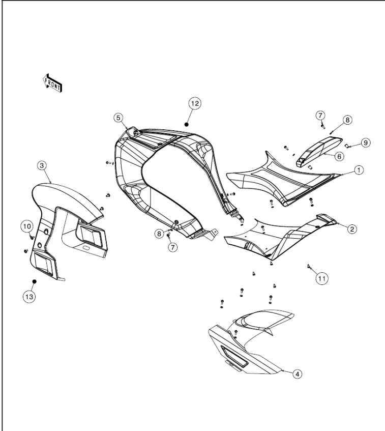
21. Fenders, seat, fuel t. cover
