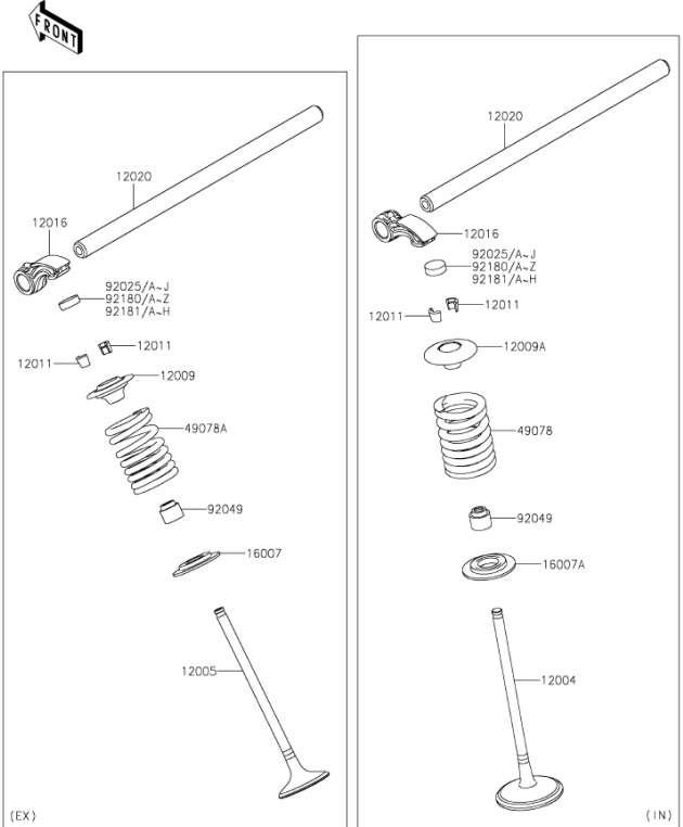
K5. Valves
