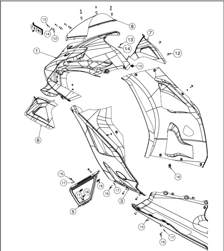
20. Front fairings
