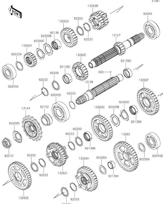
K10. Transmission
