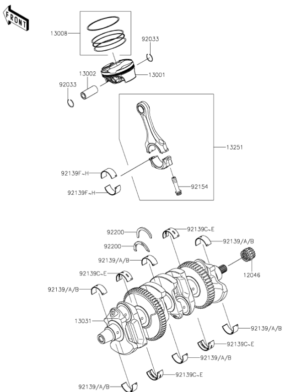
K7. Crankshaft/Pistons
