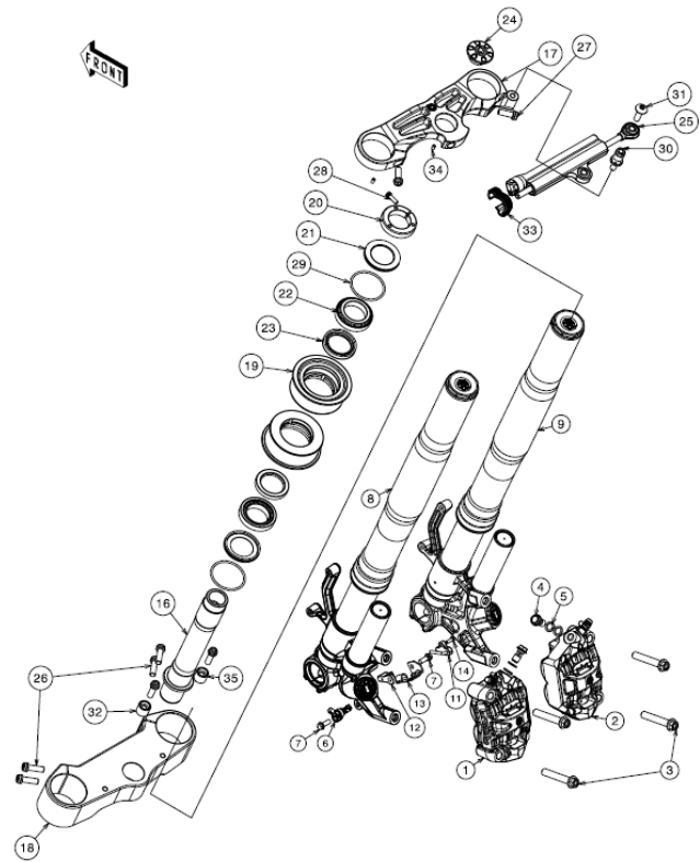
2. Frame
