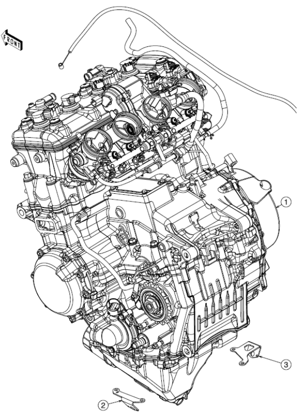
1. Engine brackets
