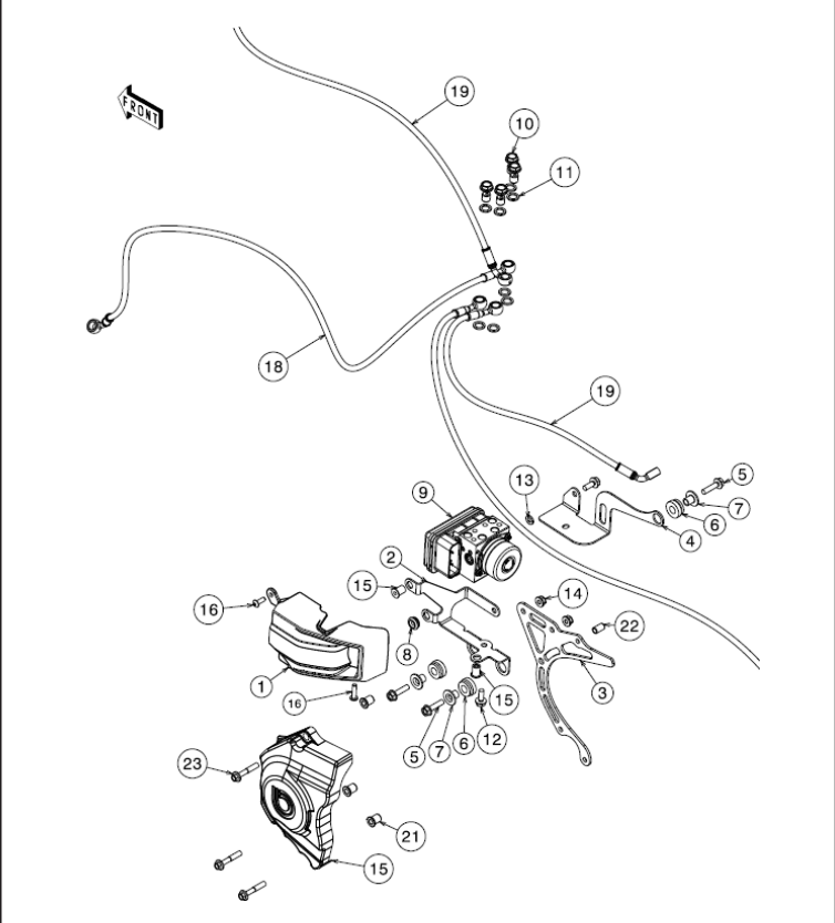
15. ABS system
