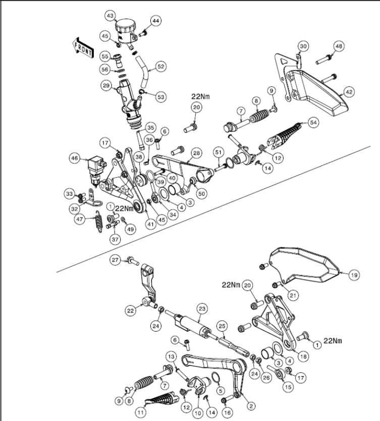
12. Footrests
