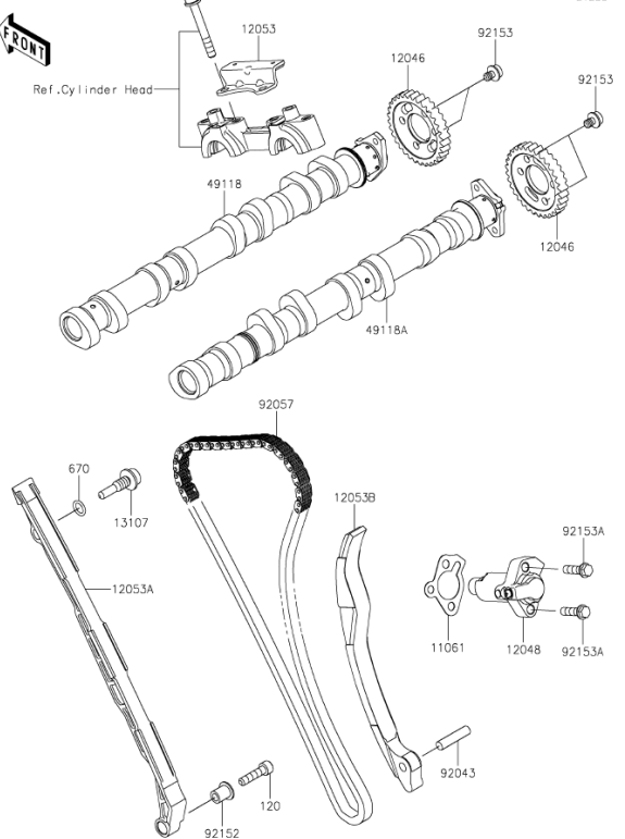
K6. Camshafts/Tensioner
