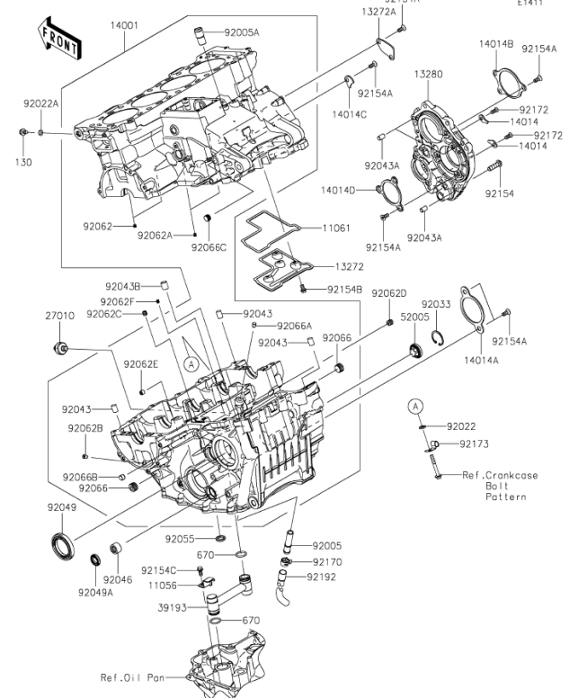
K13. Crankcase
