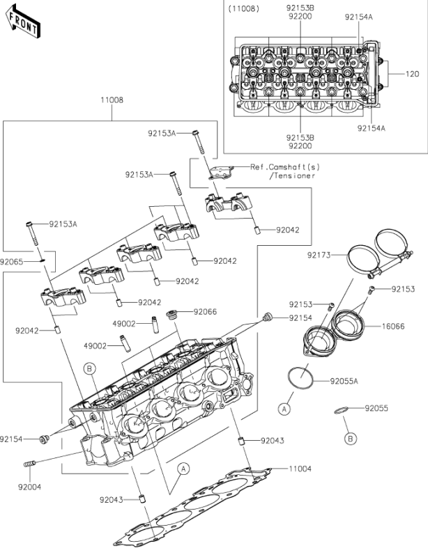
K1. Cylinder head
