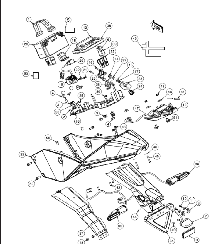
16. Tail / electronic componets
