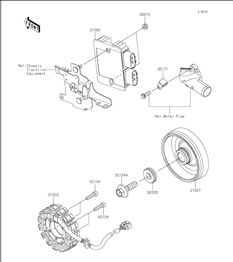
K22. Generator
