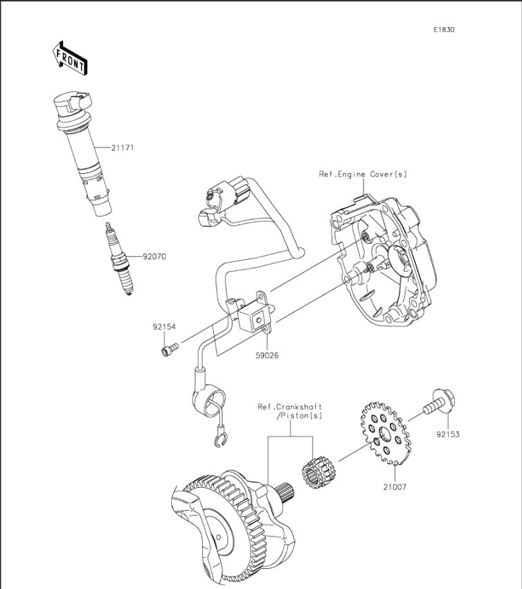
K23. Ignition system
