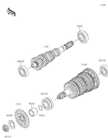
10 Transmission
