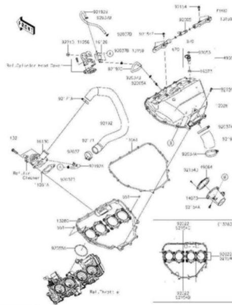
18 Air Chamber
