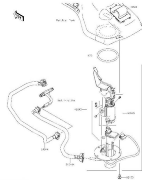
20 Fuel Pump
