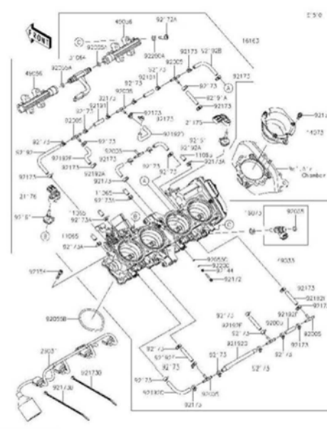
19 Throttle
