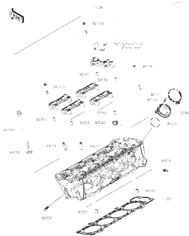
K1 Cylinder Head
