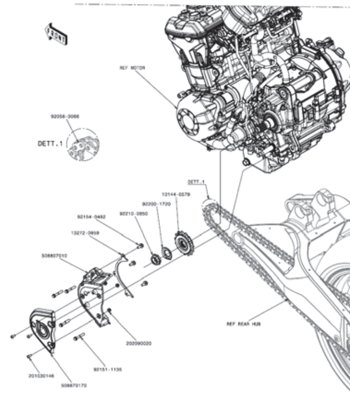
5.1 Rear wheel (sprocket hub)
