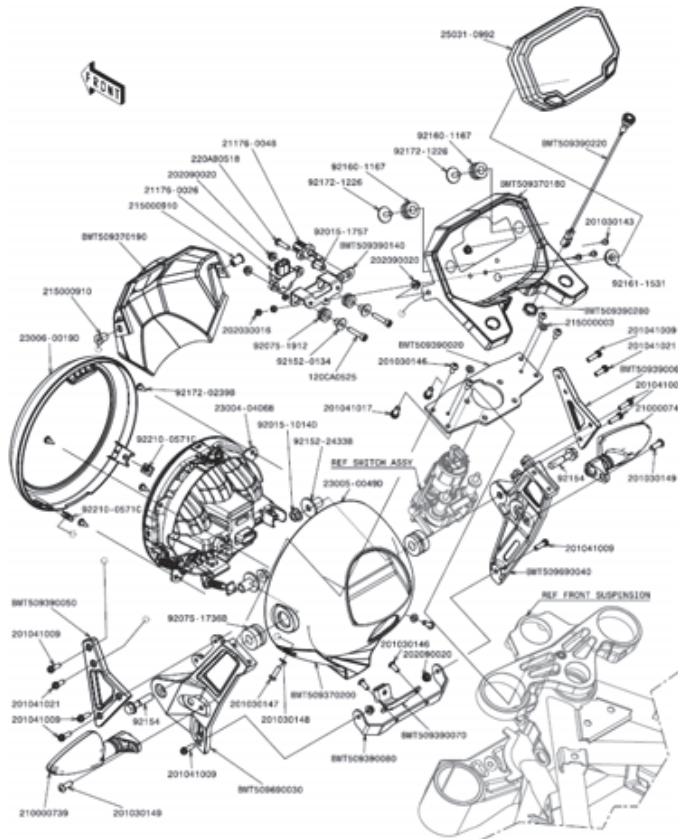
9 Front light
