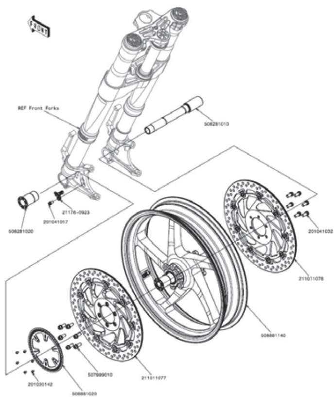
1.1 Front Wheel
