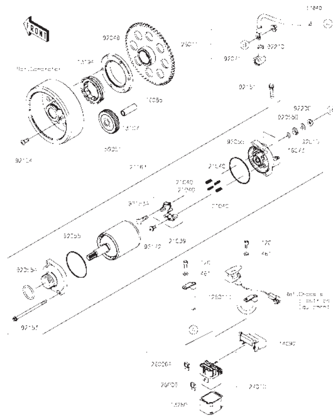
K25 Starter Motor
