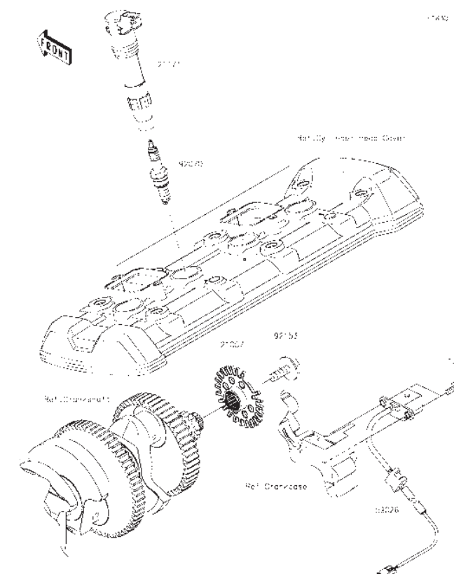
K24 Ignition System
