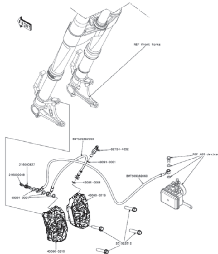
1.2 Front wheel (brake calipers)
