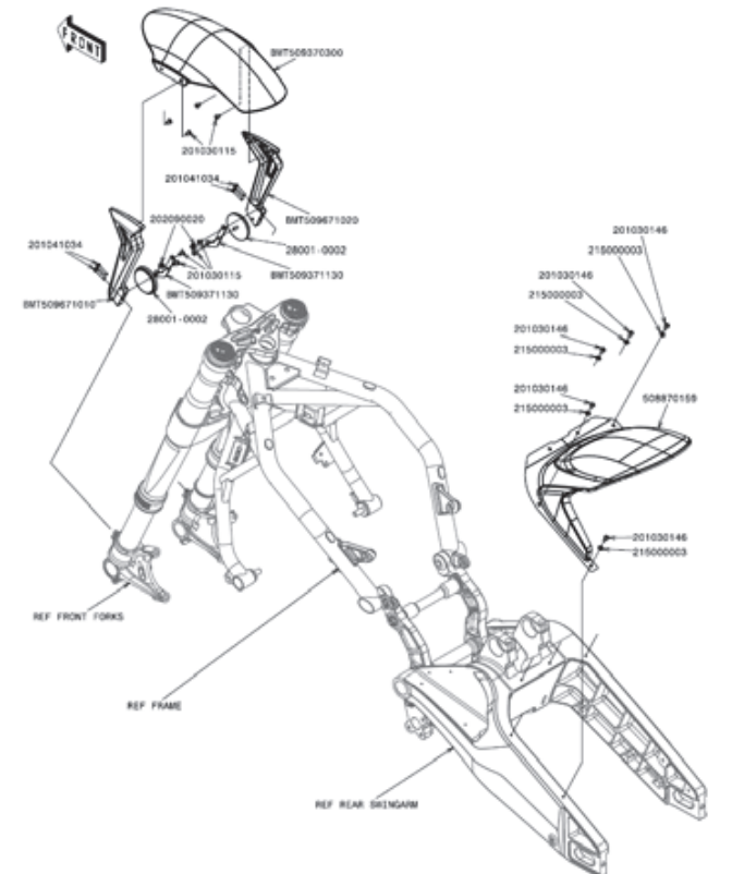
16.1 Fairings (fenders)
