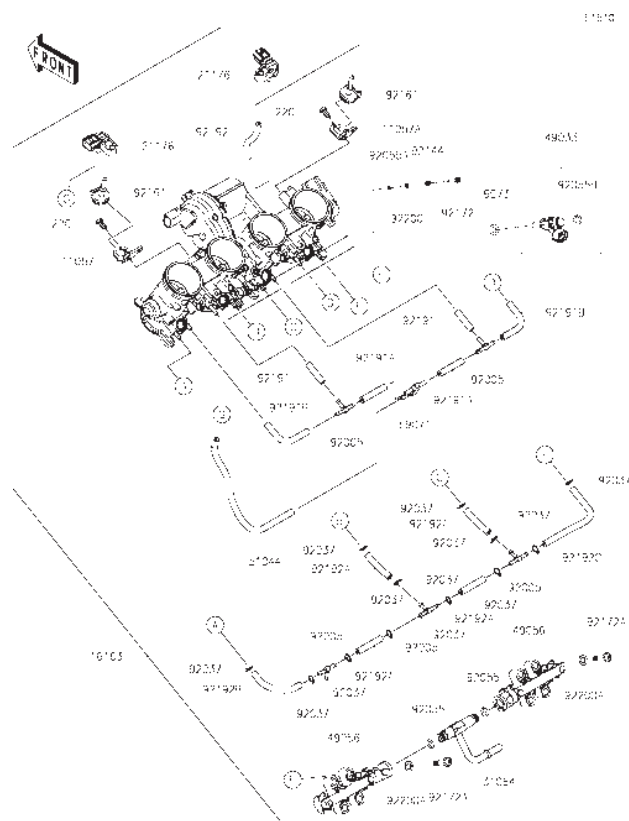
K18 Throttle
