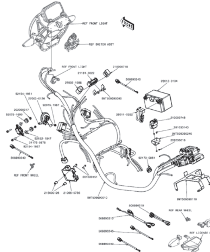
15 Electrical system
