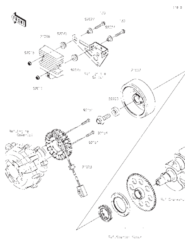
K23 Generator
