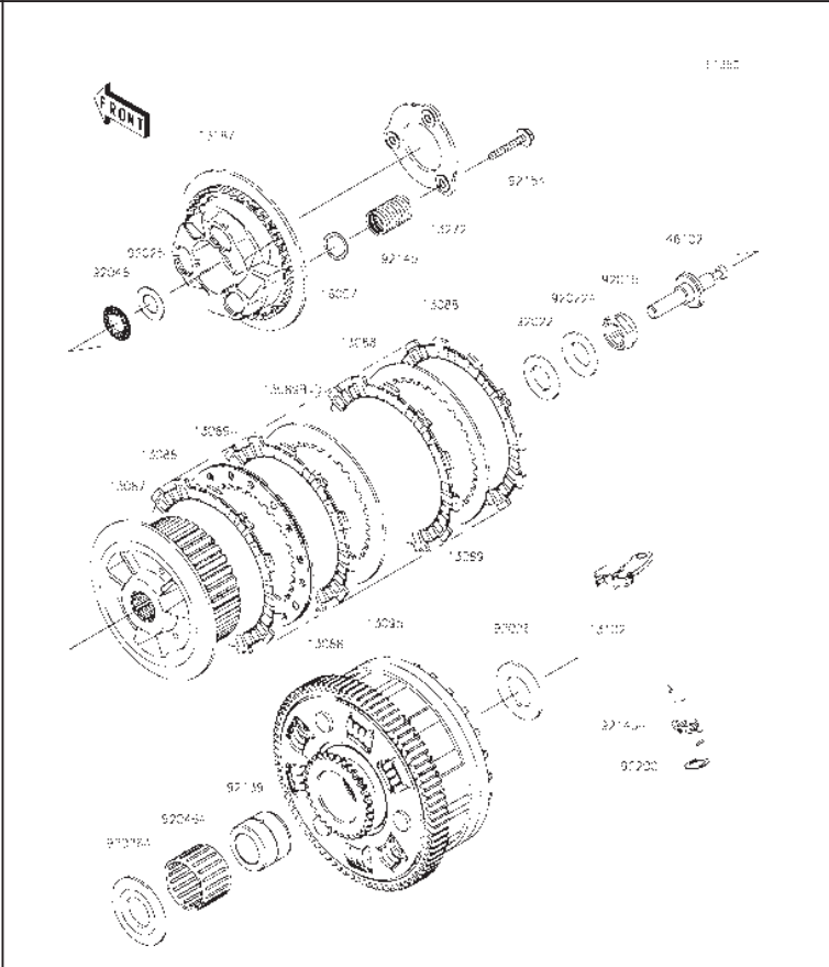
K10 Clutch
