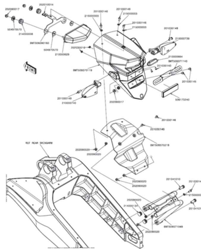
10 License plate holder
