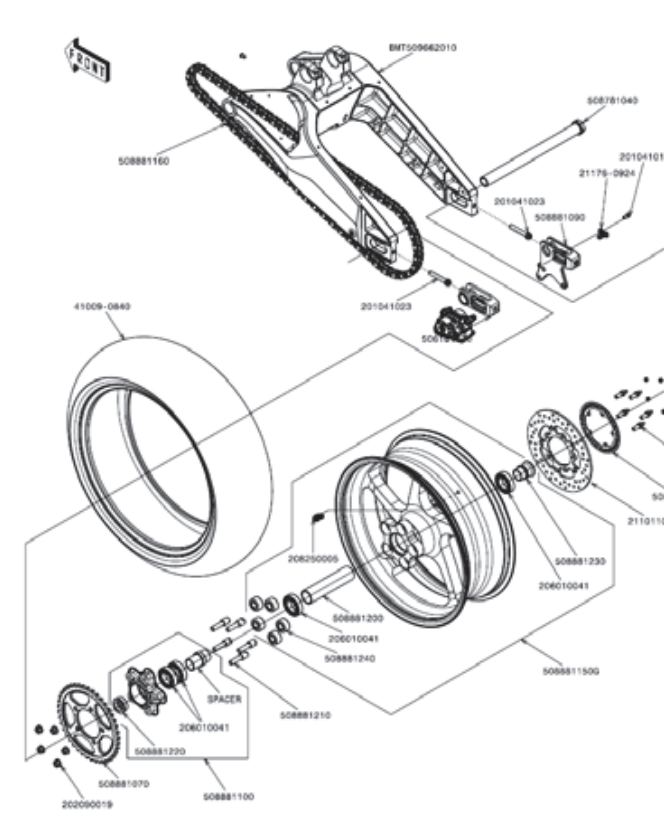
5.2 Rear wheel (wheel hub)
