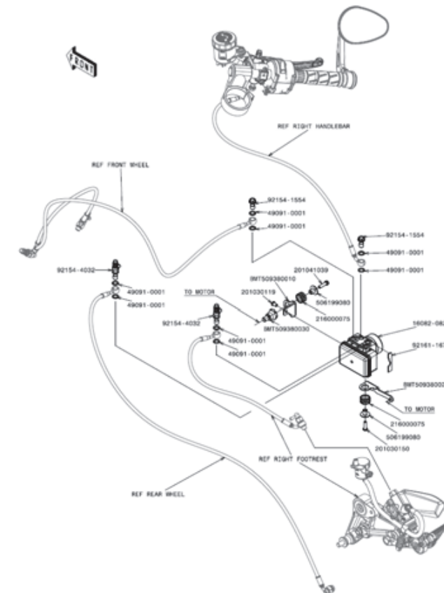
6 ABS System
