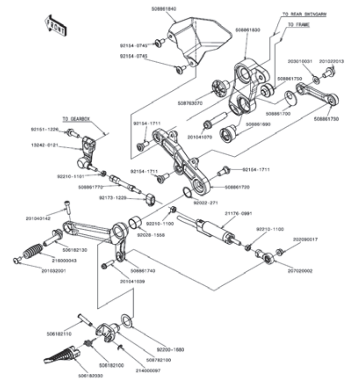
8.2 Left footrest
