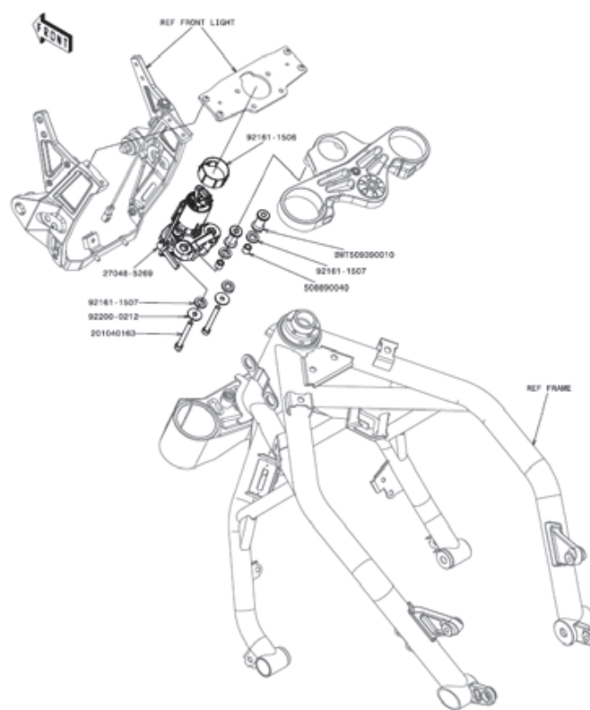
2.2 Front suspension (switch ASSY)
