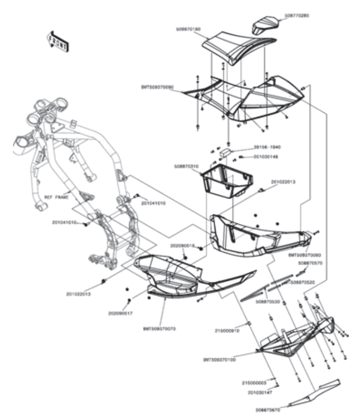
16.4 Fairings (tail & seat)
