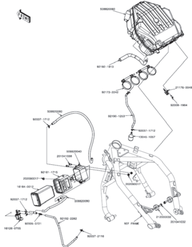
14 Airbox - fuel evaporative system
