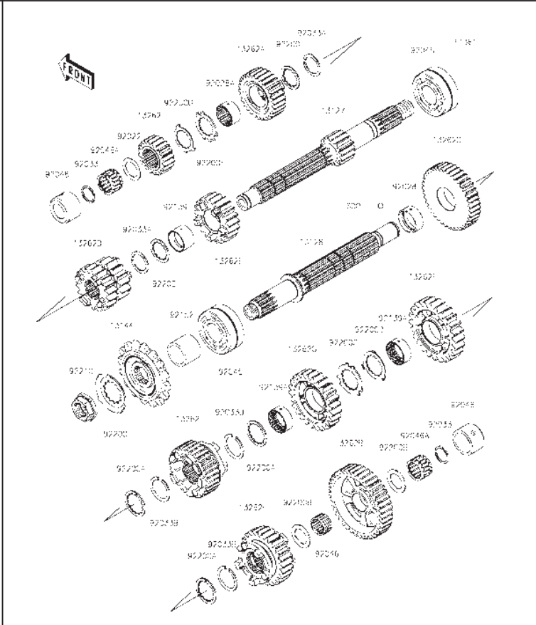
K11 Transmission
