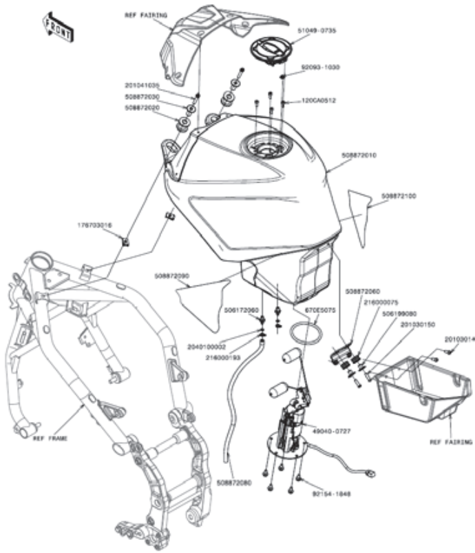
13 Fuel tank group
