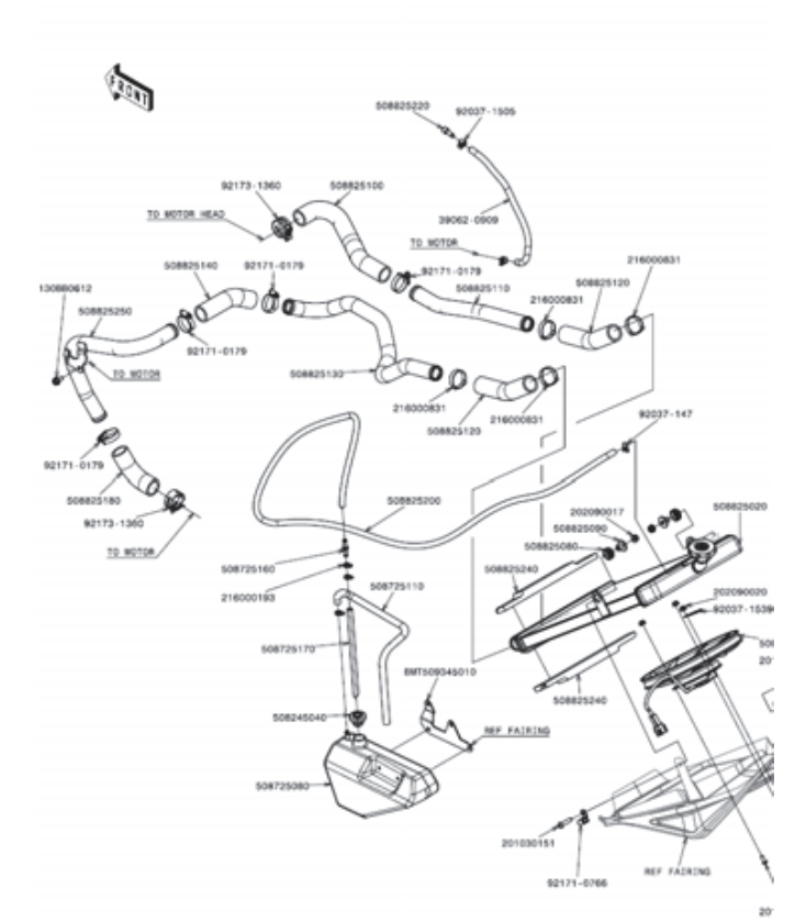
12 Cooling system
