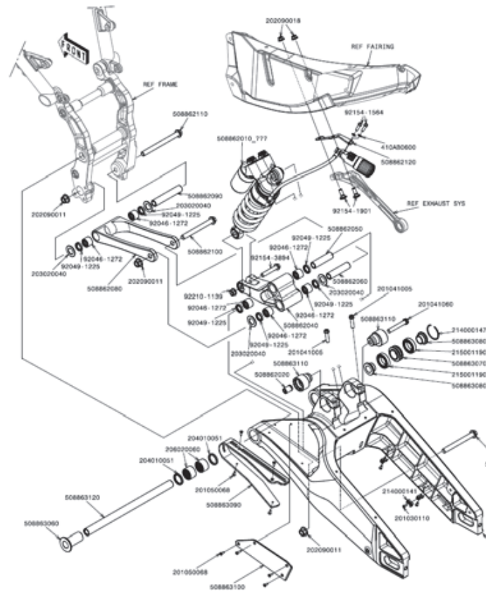
4 Rear swingarm
