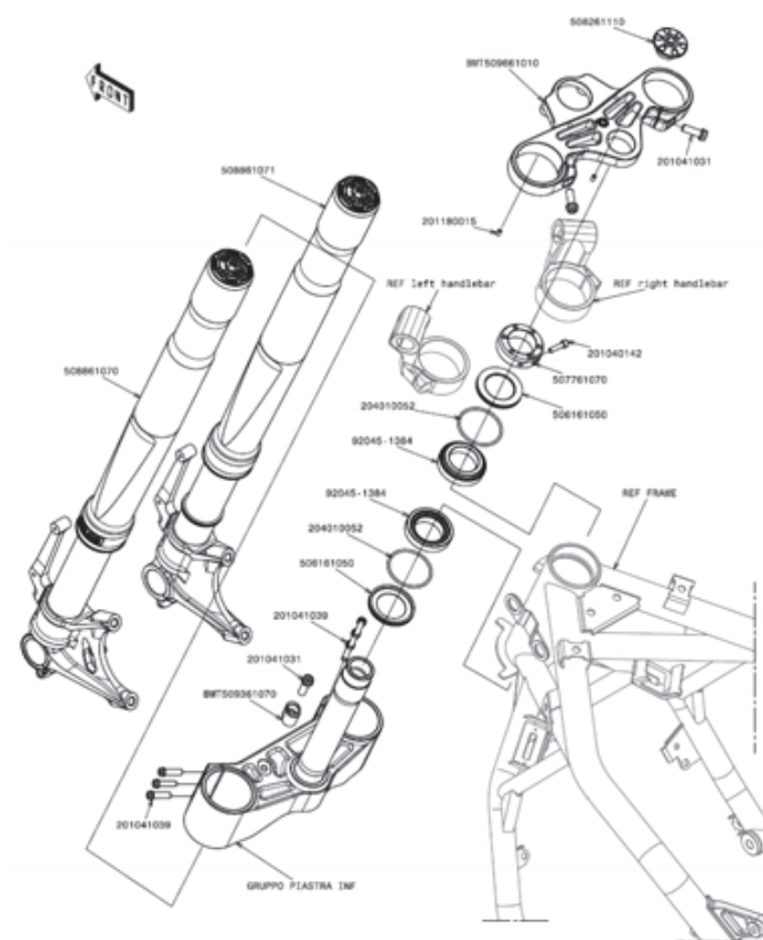
2.1 Front suspension
