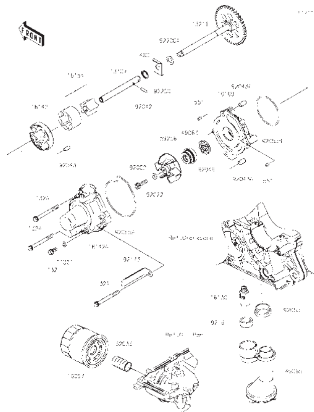
K22 Oil Pump
