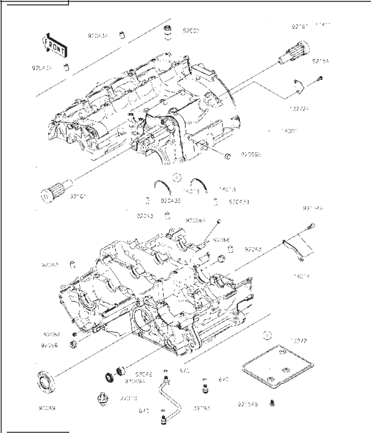
K14 Crankcase
