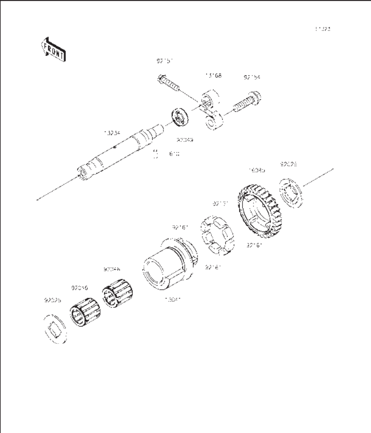
K9 Balancer
