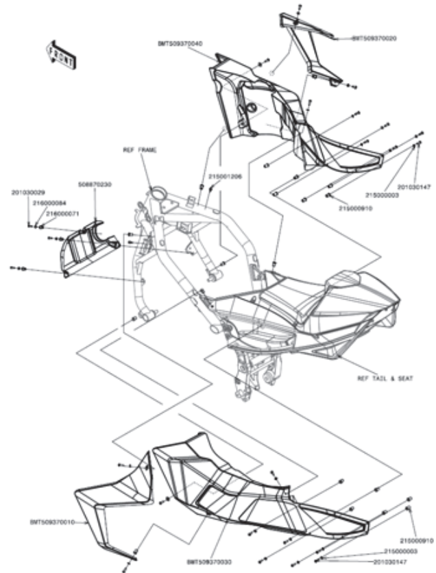
16.3 Fairings (upper parts)
